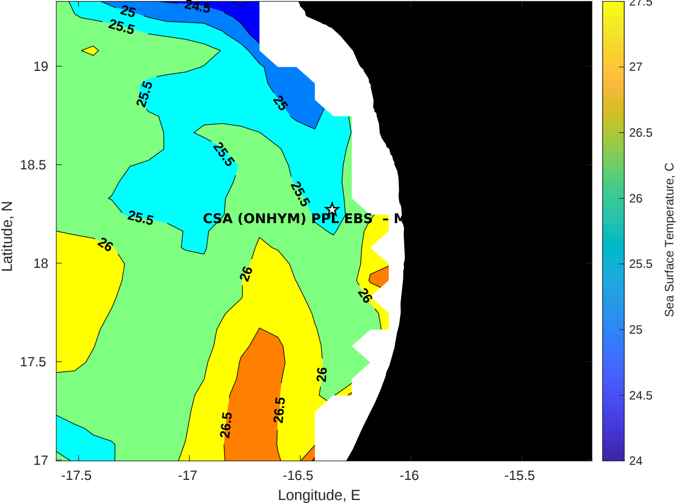
SST for CSA (ONHYM) PPL EBS - Mauritania at 03-Aug-2025 00:00:00
