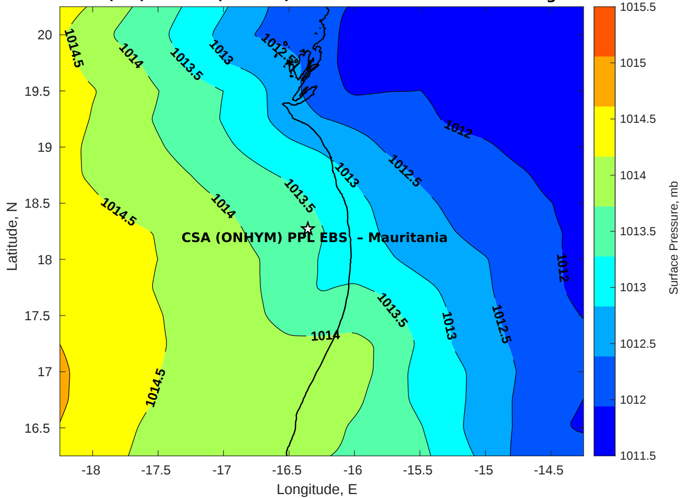
Surface Pressure (mb) for CSA (ONHYM) PPL EBS - Mauritania at 04-Aug-2025 00:00:00
