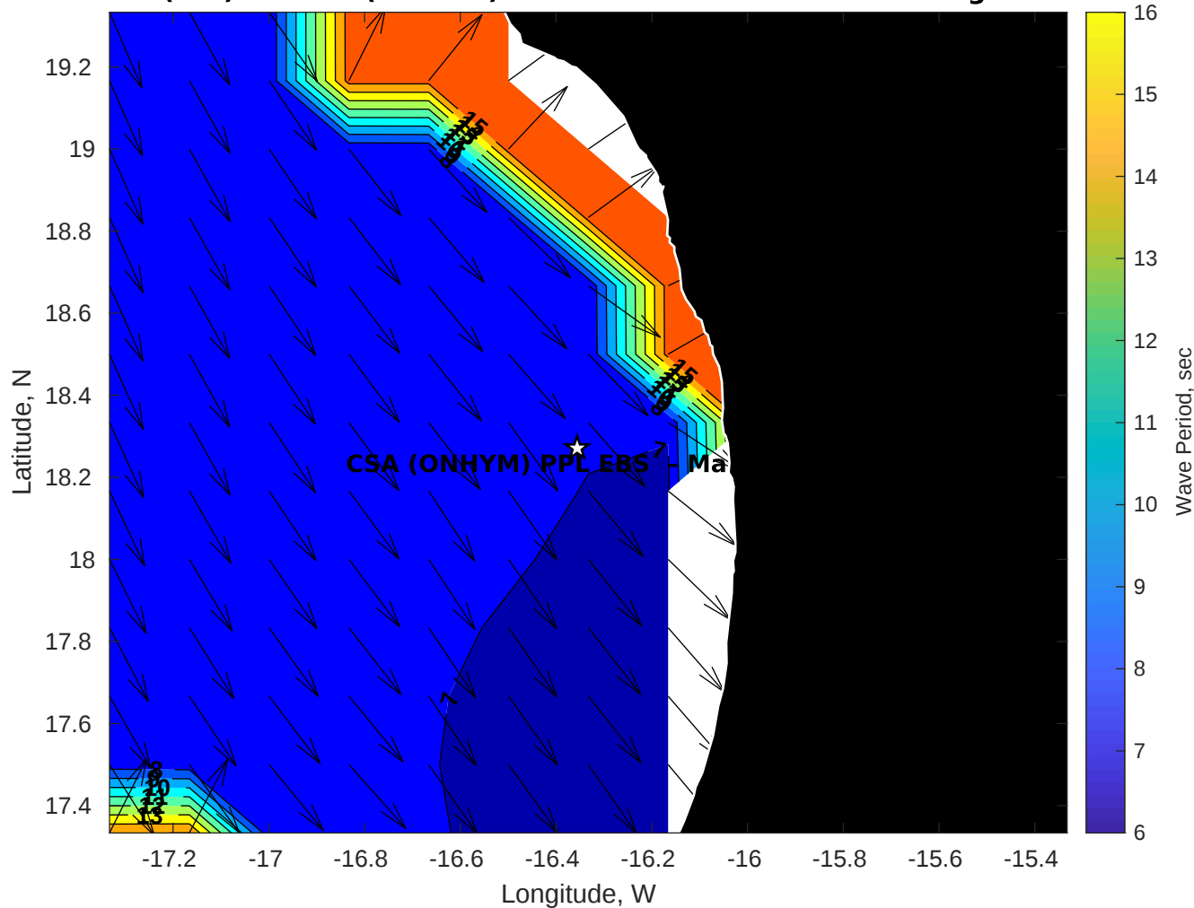
Wave Period (sec) for CSA (ONHYM) PPL EBS - Mauritania at 04-Aug-2025 09:00:00
