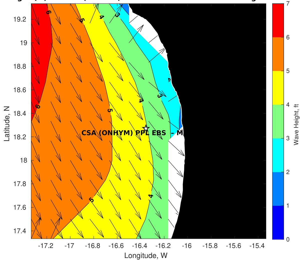
Wave Height (ft) for CSA (ONHYM) PPL EBS - Mauritania at 04-Aug-2025 09:00:00
