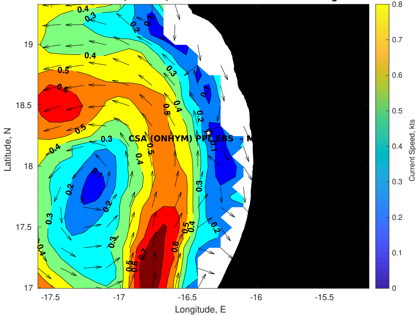
Surface Currents for CSA (ONHYM) PPL EBS - Mauritania at 03-Aug-2025 00:00:00
