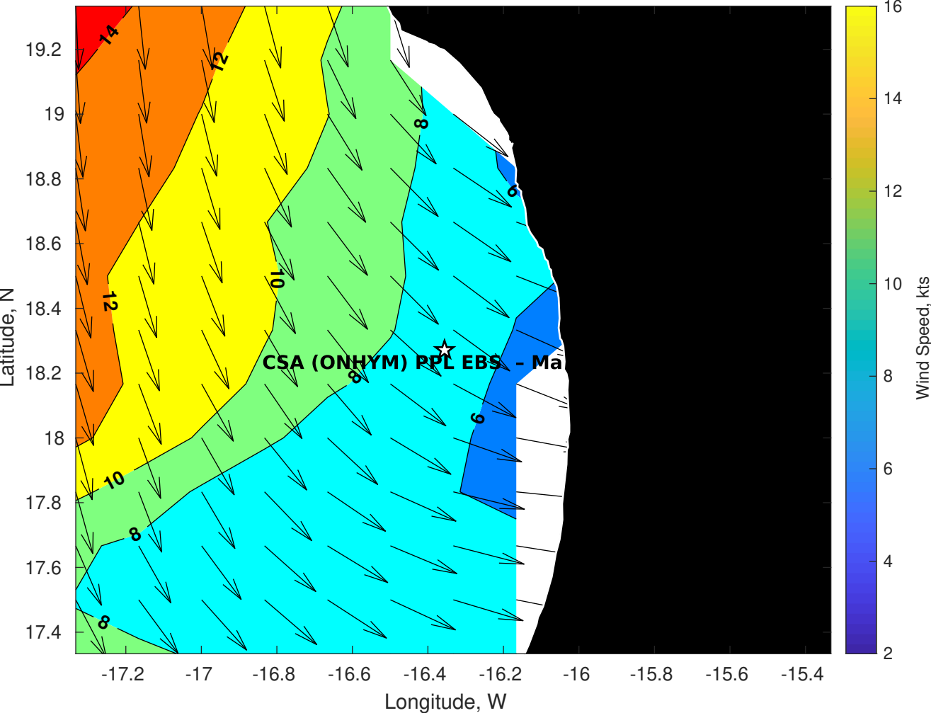
Winds (kts) for CSA (ONHYM) PPL EBS - Mauritania at 04-Aug-2025 09:00:00
