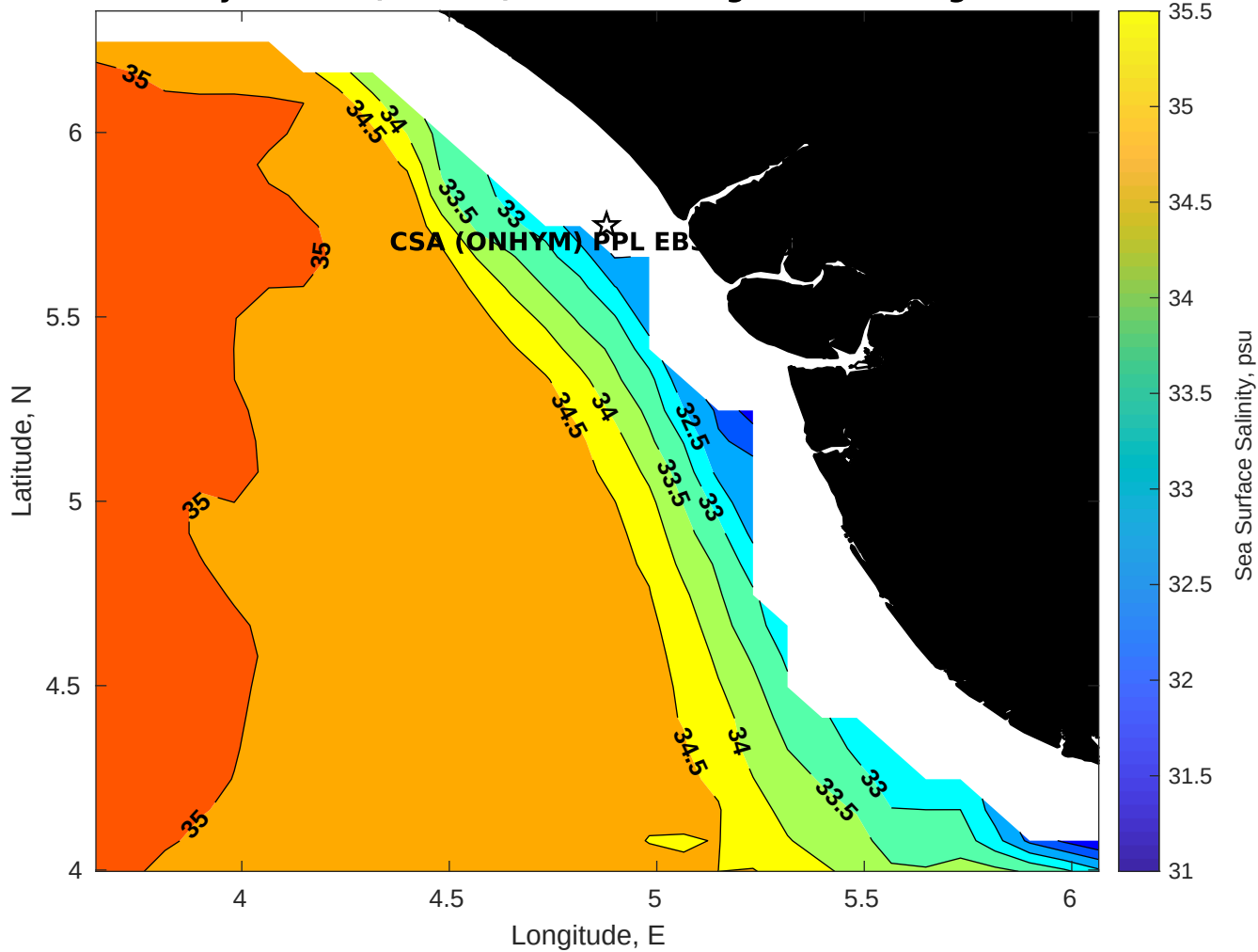
Surface Salinity for CSA (ONHYM) PPL EBS - Nigeria at 03-Aug-2025 00:00:00
