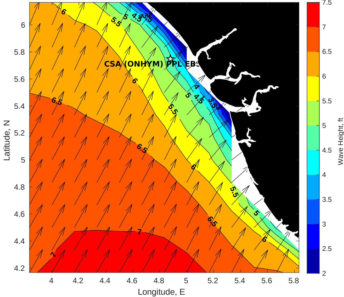
Wave Height (ft) for CSA (ONHYM) PPL EBS - Nigeria at 04-Aug-2025 09:00:00
