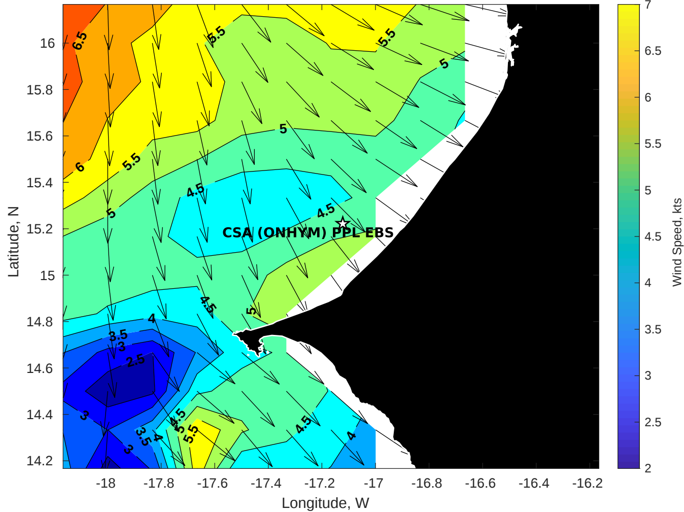
Winds (kts) for CSA (ONHYM) PPL EBS - Senegal at 04-Aug-2025 09:00:00
