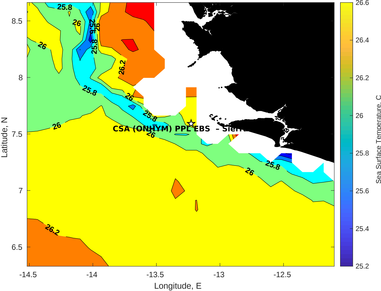
SST for CSA (ONHYM) PPL EBS - Sierra Leone at 03-Aug-2025 00:00:00
