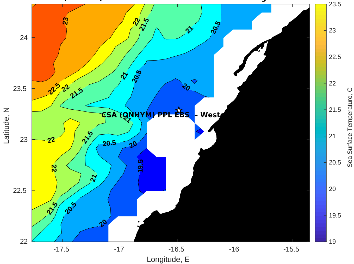
SST for CSA (ONHYM) PPL EBS - Western Sahara at 03-Aug-2025 00:00:00
