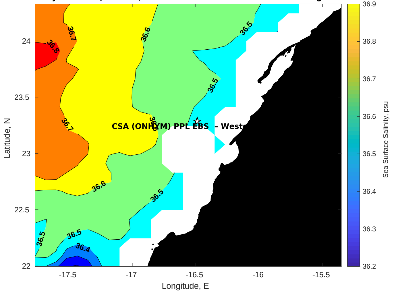
Surface Salinity for CSA (ONHYM) PPL EBS - Western Sahara at 03-Aug-2025 00:00:00
