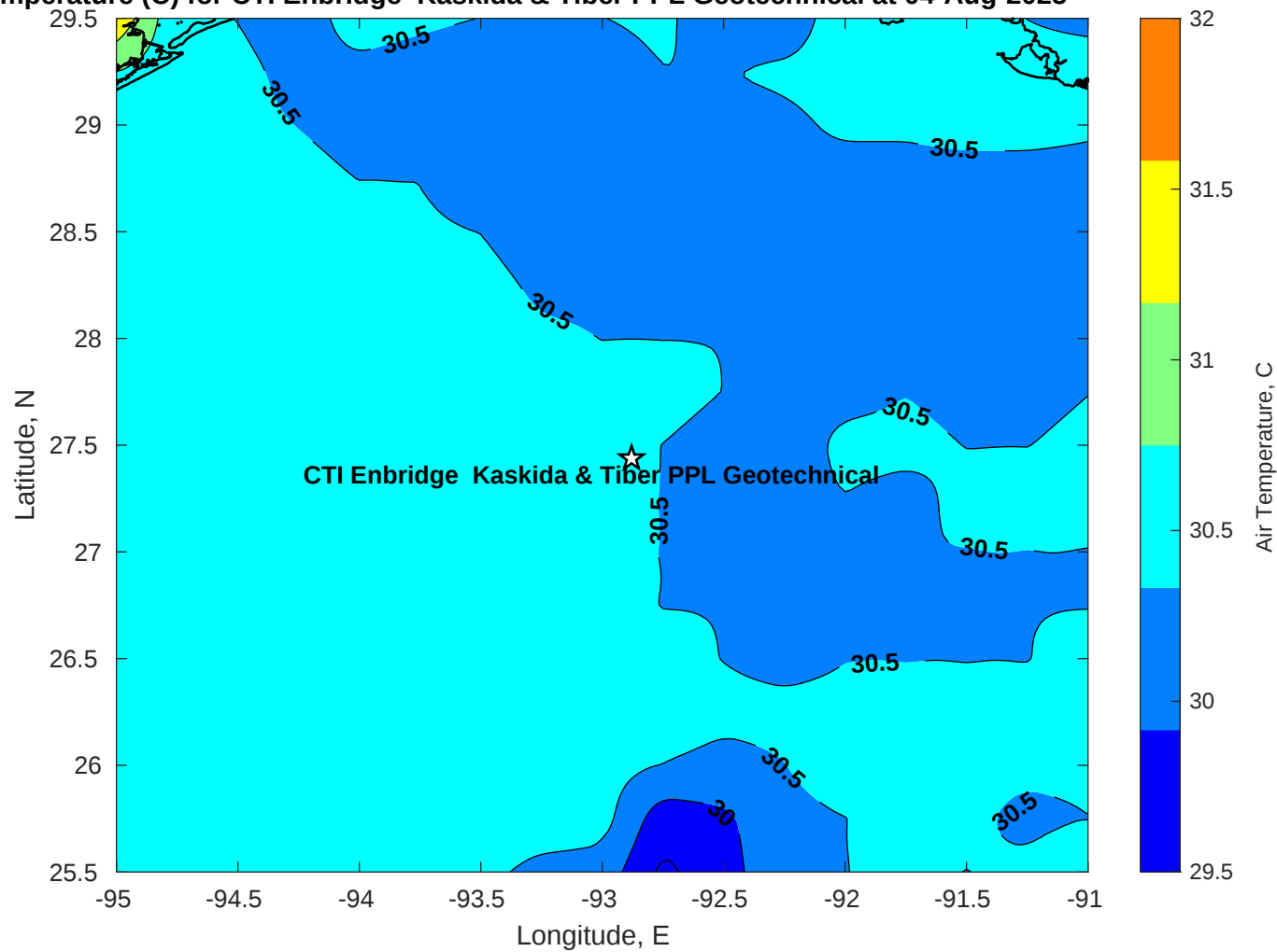
Air Temperature (C) for CTI Enbridge Kaskida & Tiber PPL Geotechnical at 04-Aug-2025
