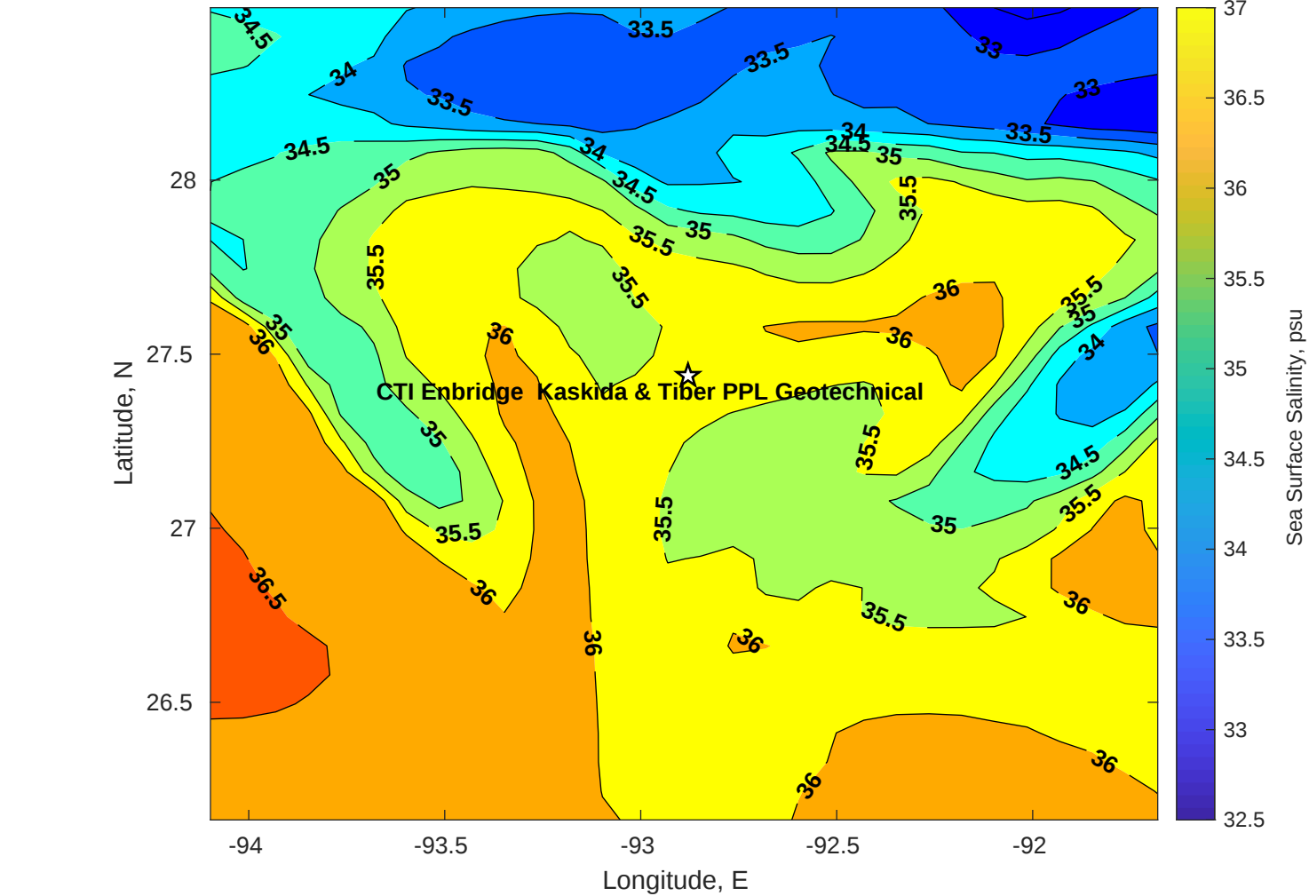
Surface Salinity for CTI Enbridge Kaskida & Tiber PPL Geotechnical at 03-Aug-2025 00:00:00
