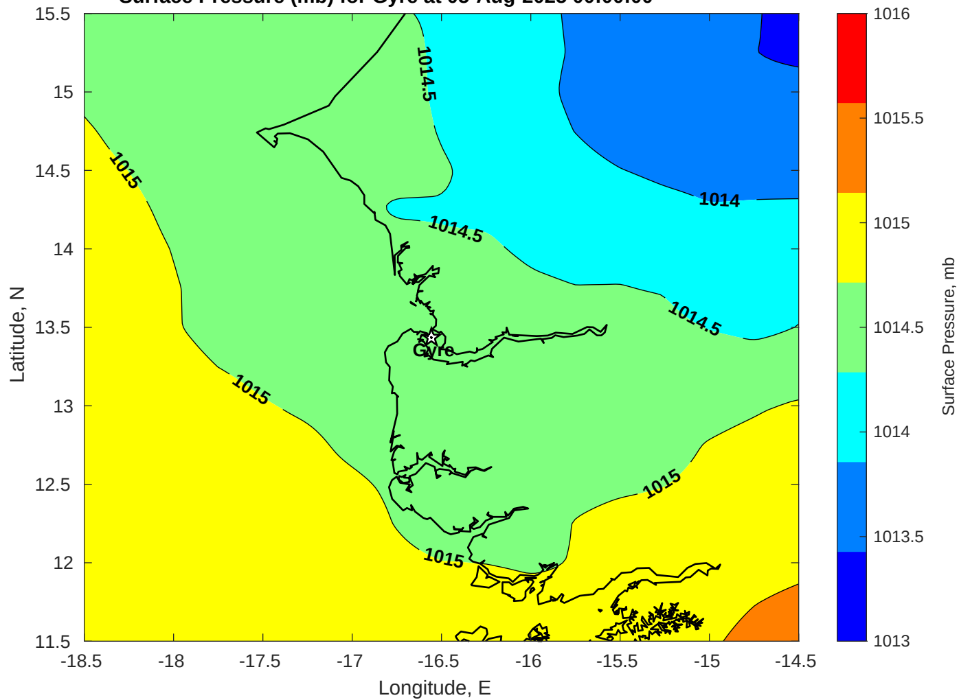
Surface Pressure (mb) for Gyre at 05-Aug-2025 00:00:00
