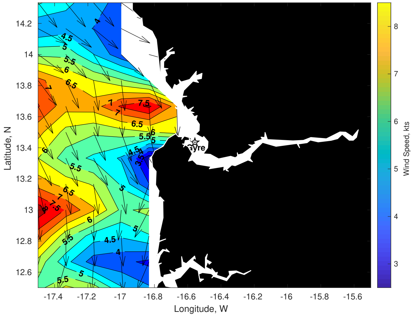
Winds (kts) for Gyre at 04-Aug-2025 09:00:00
