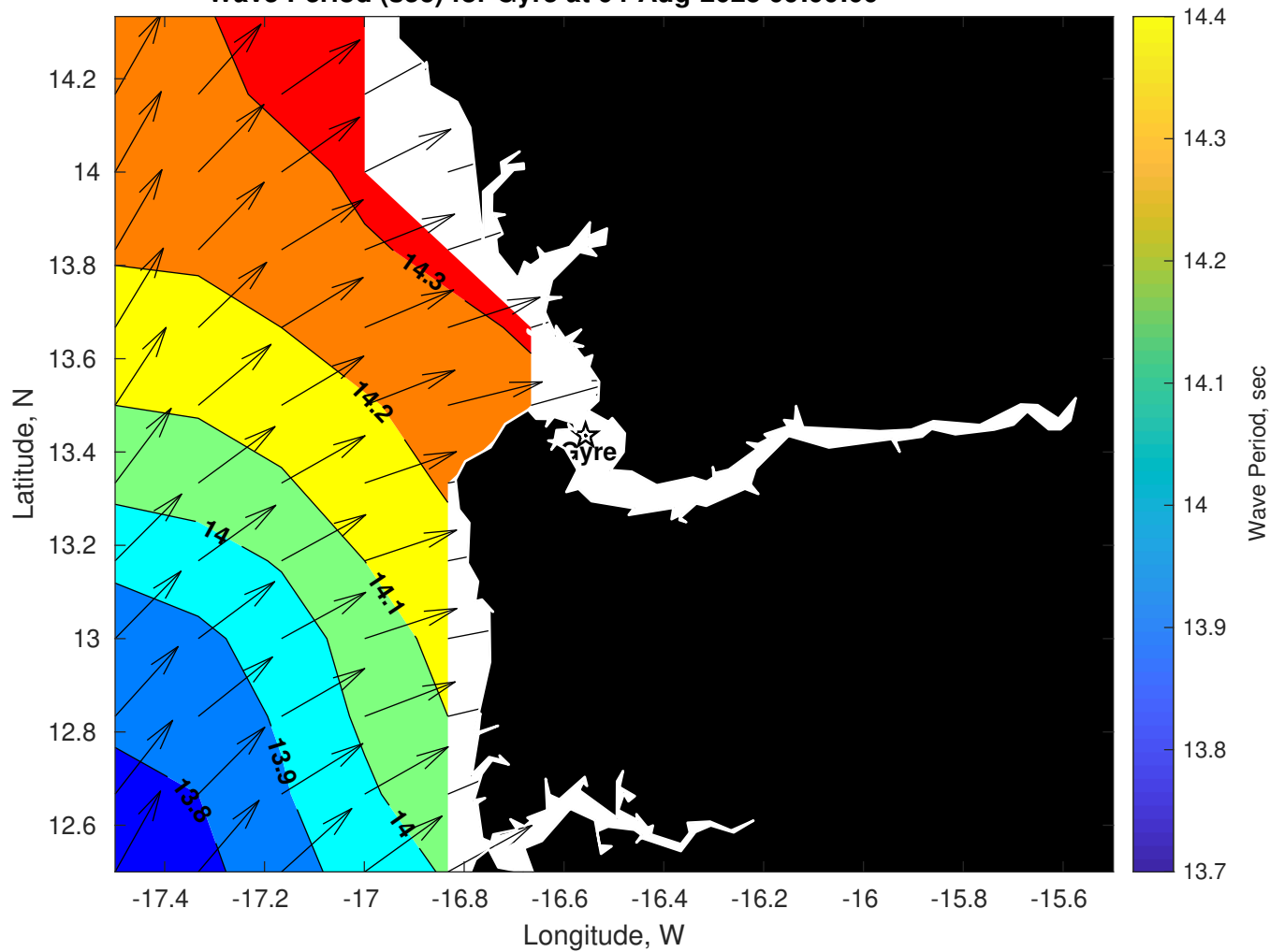
Wave Period (sec) for Gyre at 04-Aug-2025 09:00:00
