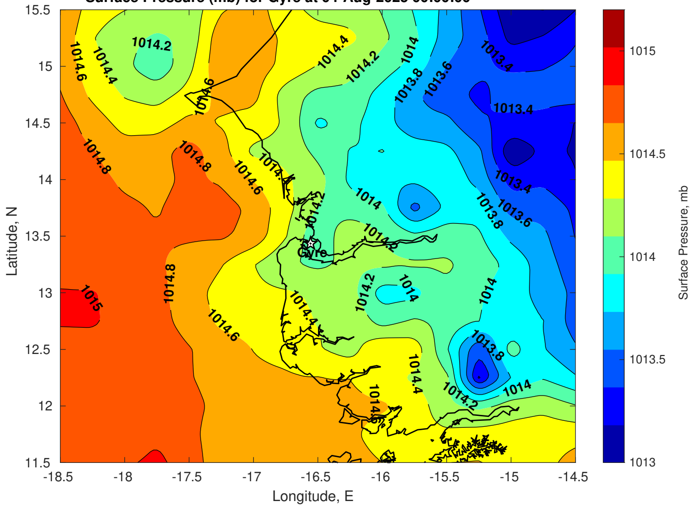
Surface Pressure (mb) for Gyre at 04-Aug-2025 00:00:00
