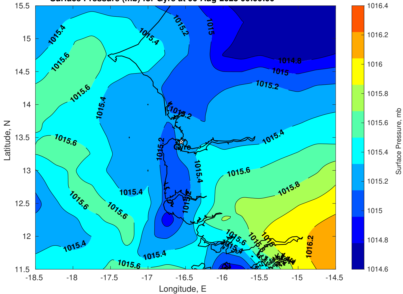
Surface Pressure (mb) for Gyre at 06-Aug-2025 00:00:00
