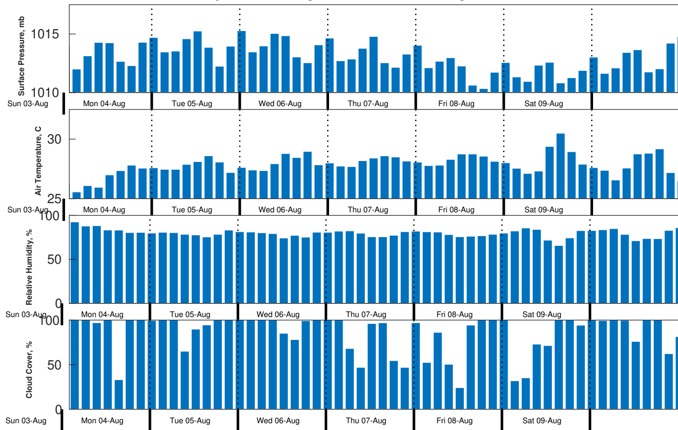
Met Forecast for Gyre from 03-Aug-2025 23:00:00 to 10-Aug-2025 23:00:00
