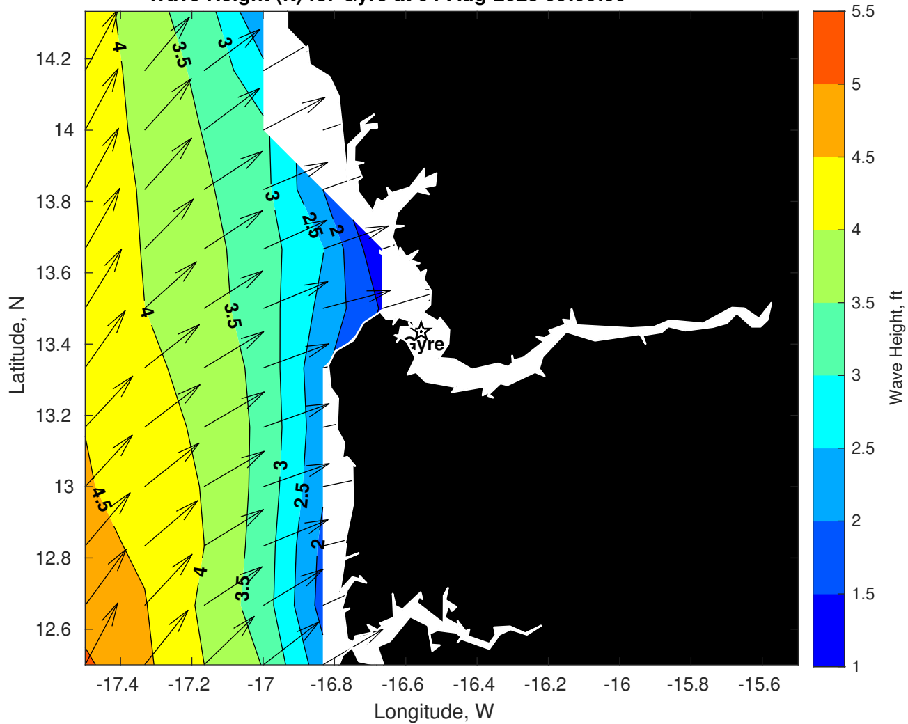
Wave Height (ft) for Gyre at 04-Aug-2025 09:00:00
