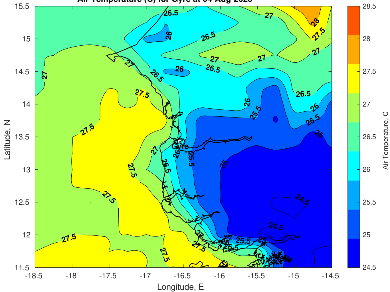
Air Temperature (C) for Gyre at 04-Aug-2025
