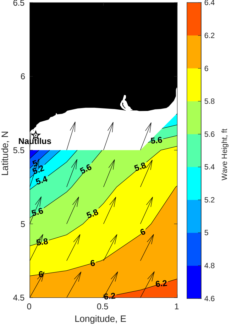
Wave Height (ft) for Nautilus at 04-Aug-2025 09:00:00
