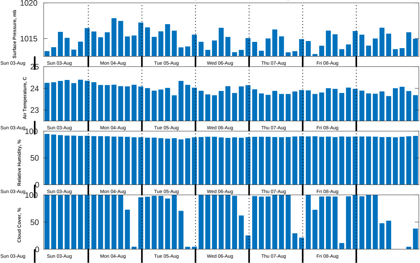
Met Forecast for Nautilus from 04-Aug-2025 00:00:00 to 11-Aug-2025 00:00:00
