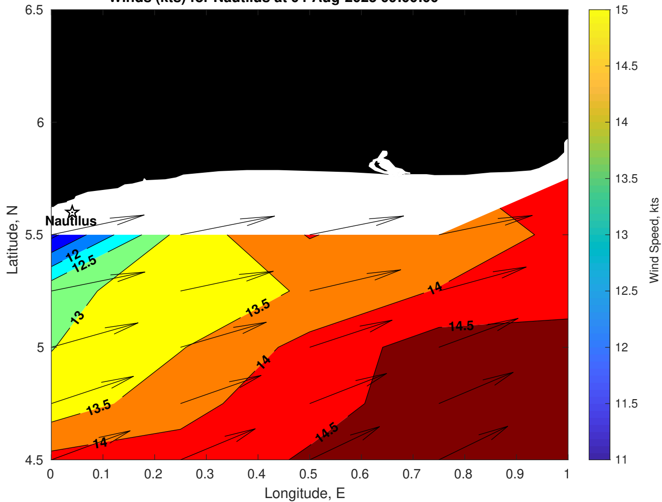
Winds (kts) for Nautilus at 04-Aug-2025 09:00:00
