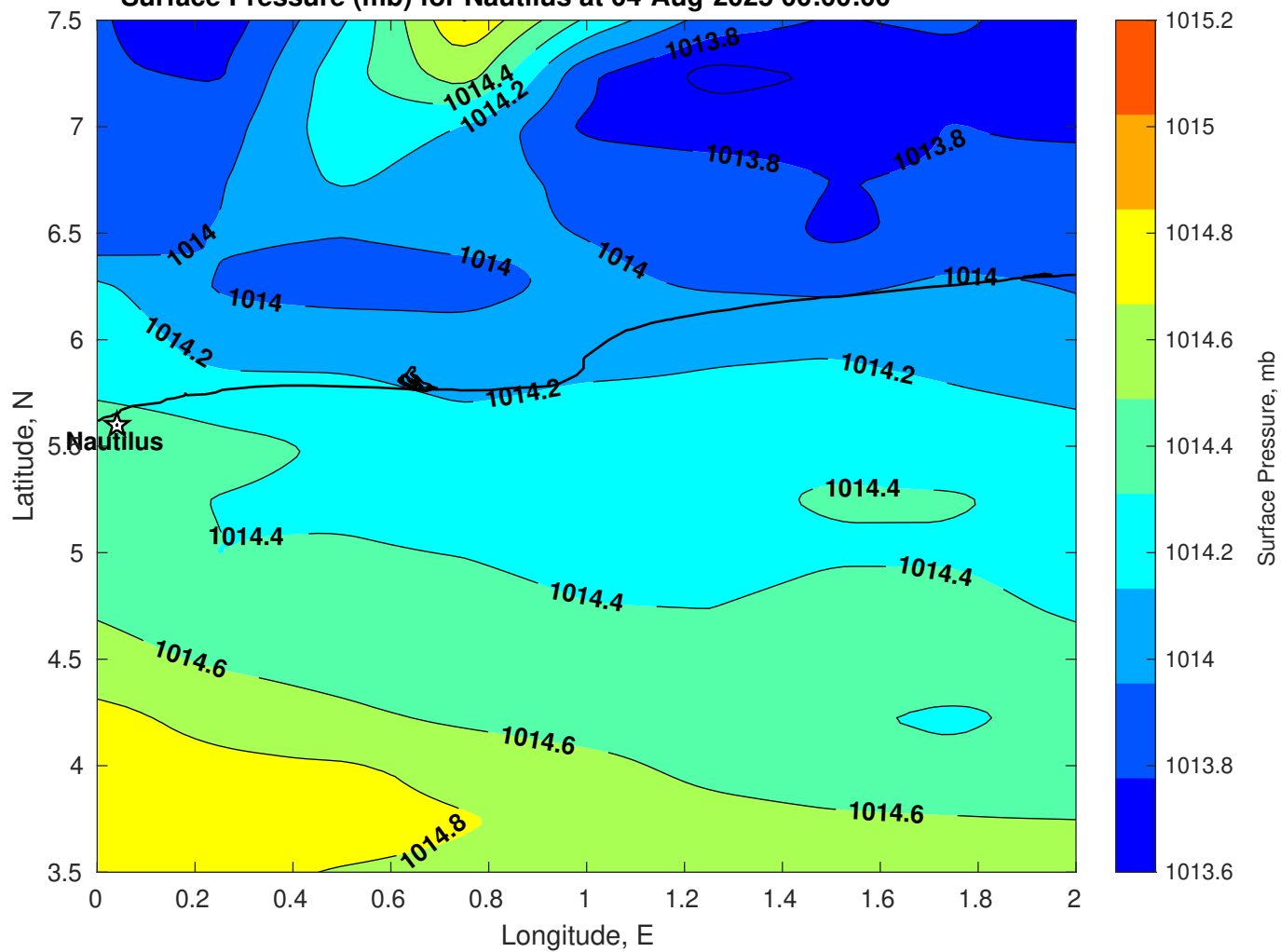
Surface Pressure (mb) for Nautilus at 04-Aug-2025 00:00:00
