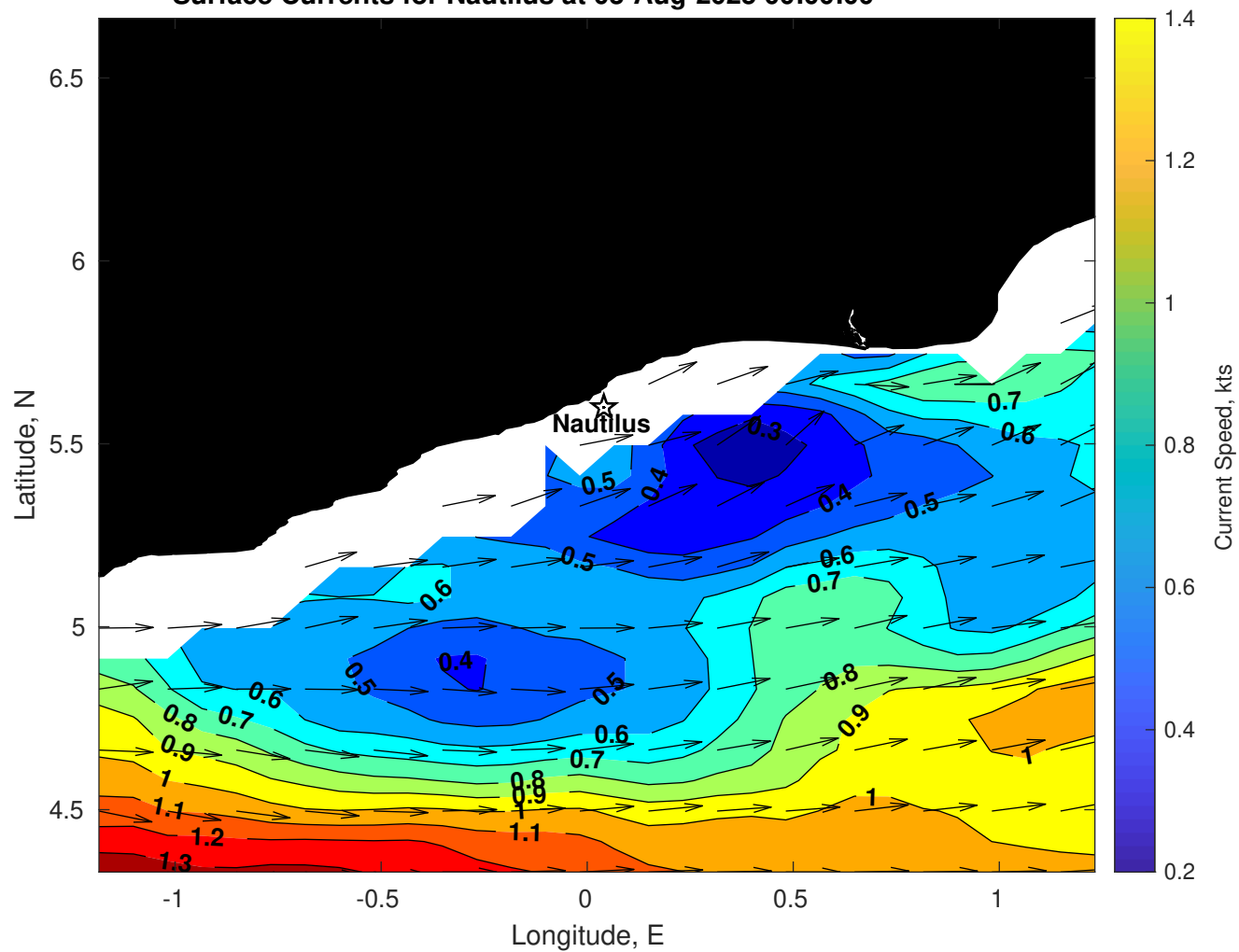
Surface Currents for Nautilus at 03-Aug-2025 00:00:00
