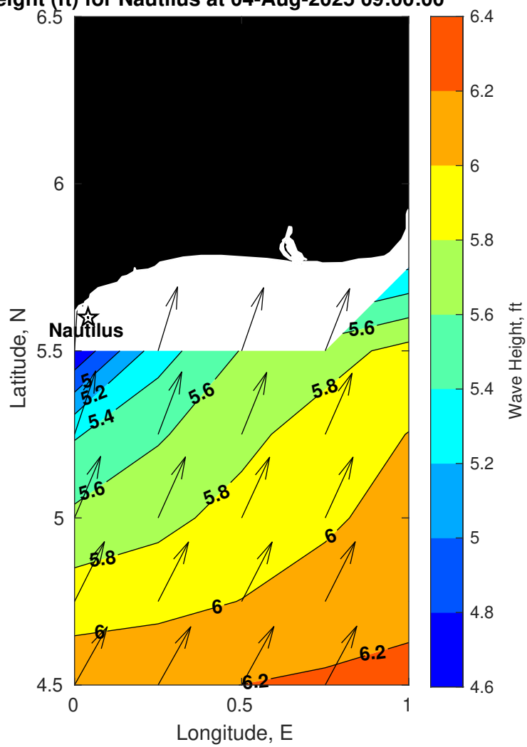
Wave Height (ft) for Nautilus at 04-Aug-2025 09:00:00
