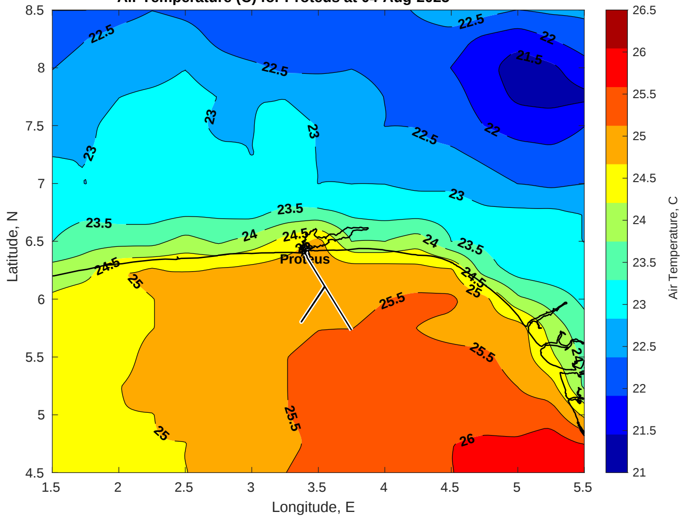
Air Temperature (C) for Proteus at 04-Aug-2025
