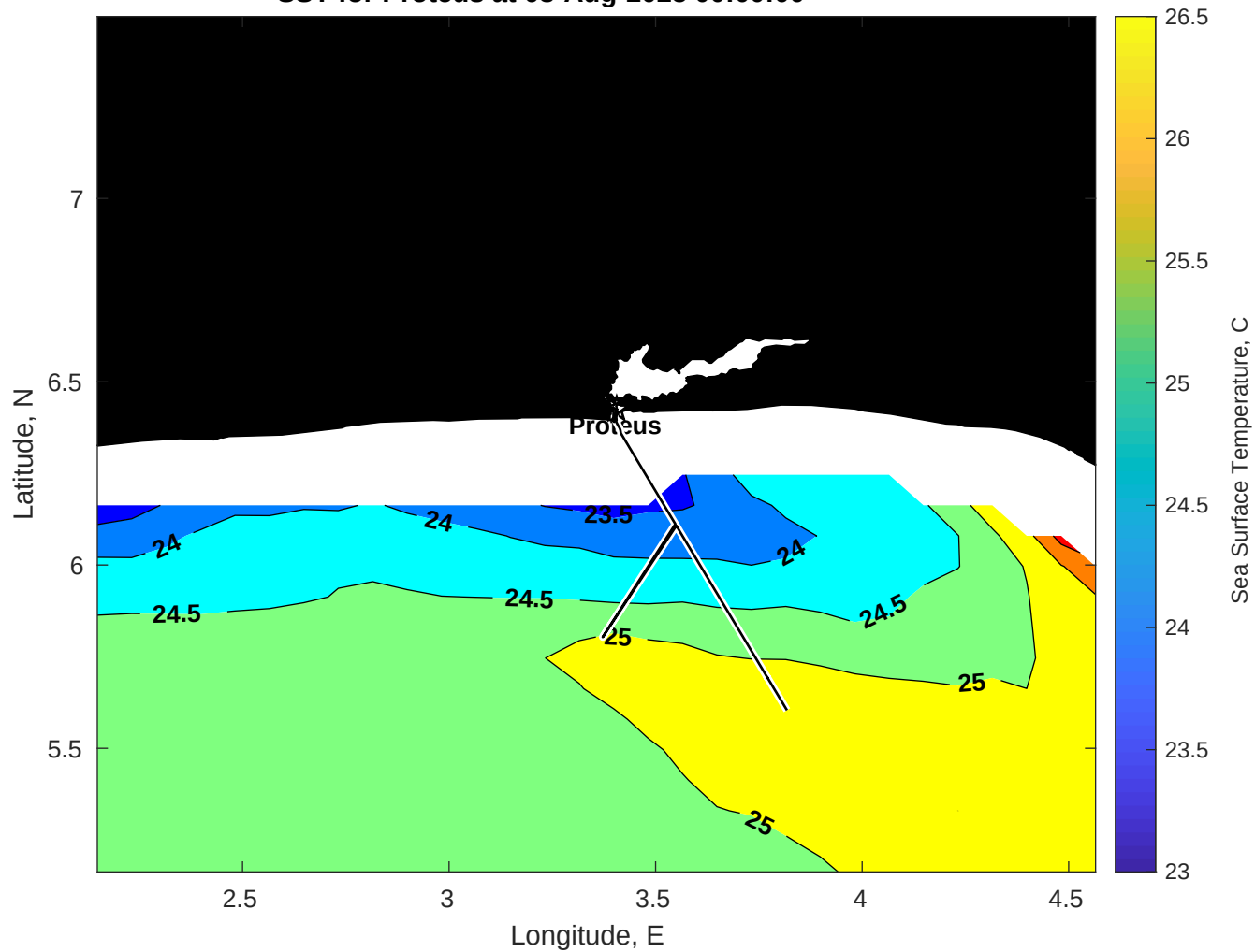
SST for Proteus at 03-Aug-2025 00:00:00
