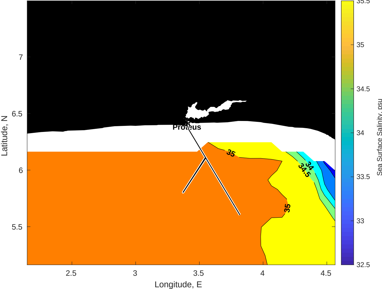
Surface Salinity for Proteus at 03-Aug-2025 00:00:00
