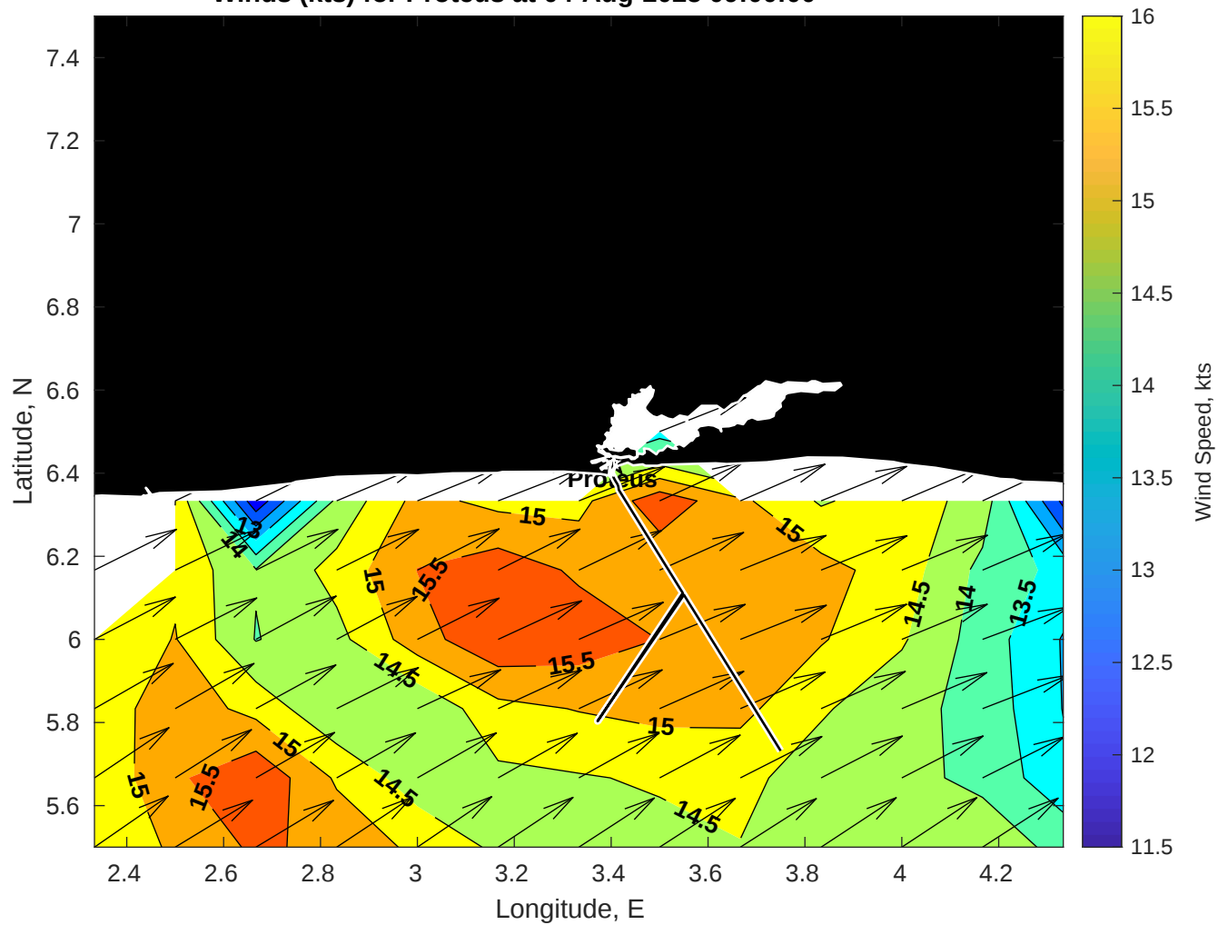
Winds (kts) for Proteus at 04-Aug-2025 09:00:00
