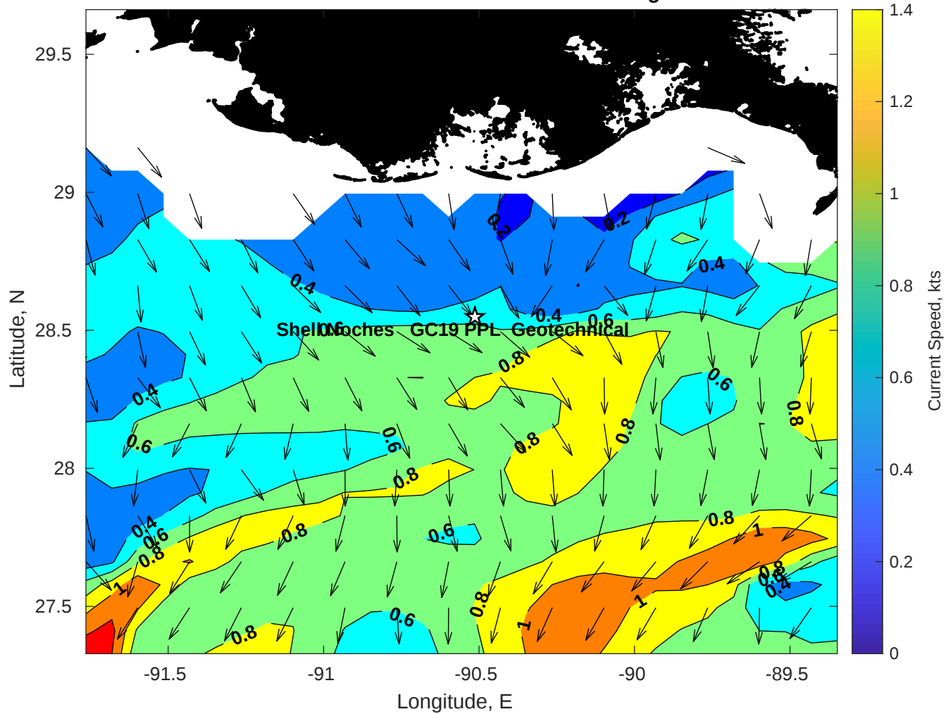
Surface Currents for Shell Noches GC19 PPL Geotechnical at 03-Aug-2025 00:00:00
