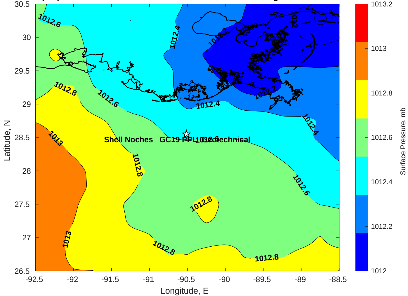
Surface Pressure (mb) for Shell Noches GC19 PPL Geotechnical at 04-Aug-2025 00:00:00
