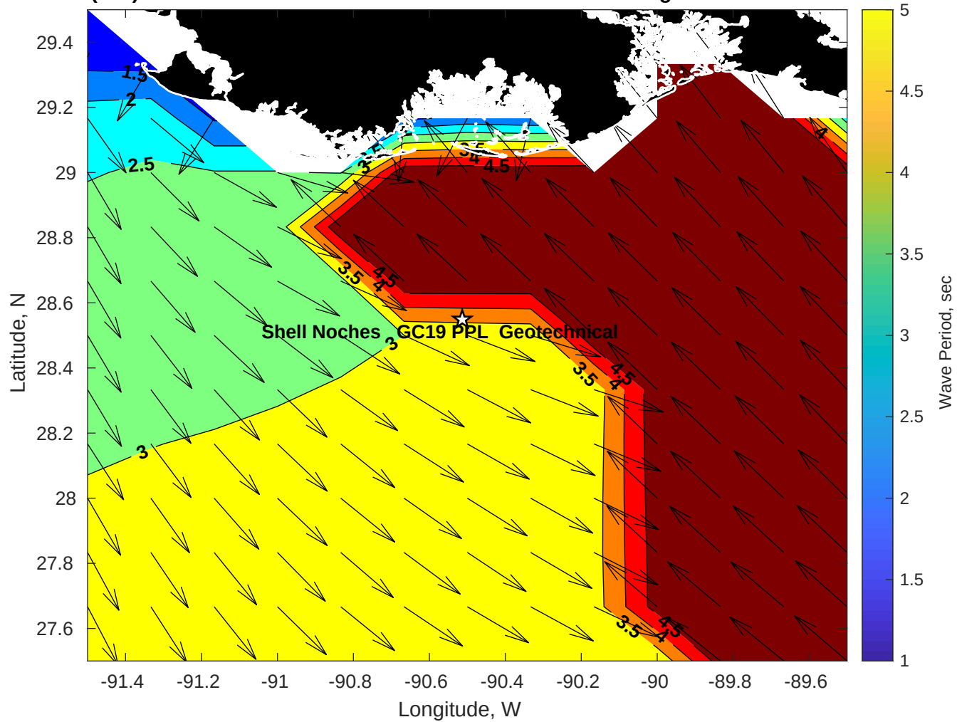
Wave Period (sec) for Shell Noches GC19 PPL Geotechnical at 04-Aug-2025 09:00:00
