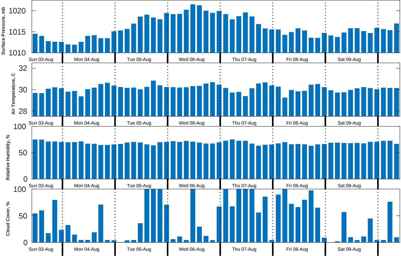
Met Forecast for Shell Noches GC19 PPL Geotechnical from 03-Aug-2025 12:00:00 to 10-Aug-2025 12:00:00
