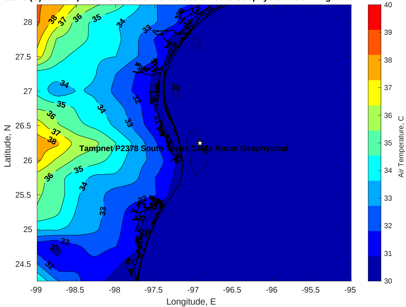
Air Temperature (C) for Tampnet P2378 South Texas Cable Route Geophysical at 04-Aug-2025
