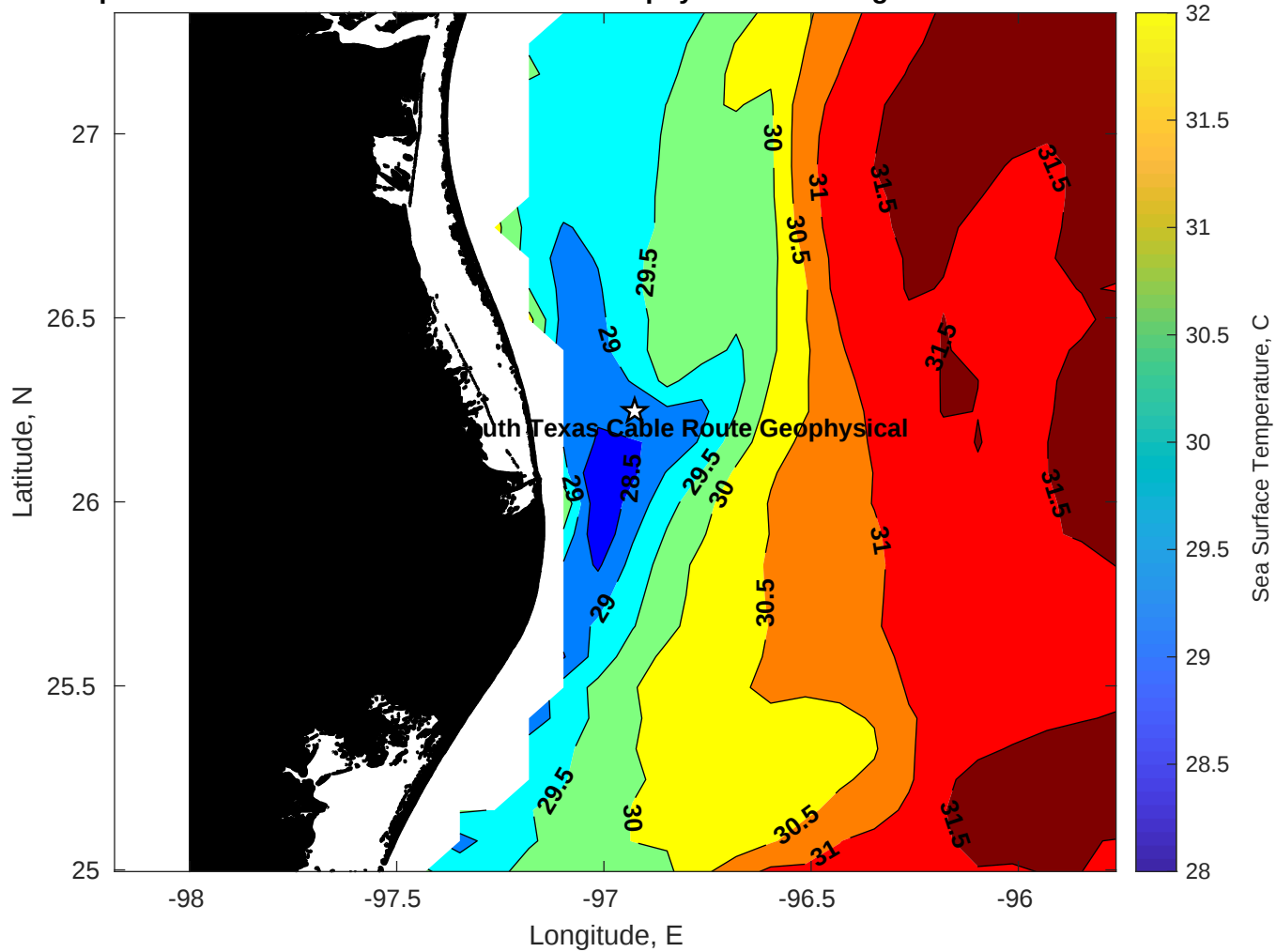
SST for Tampnet P2378 South Texas Cable Route Geophysical at 03-Aug-2025 00:00:00
