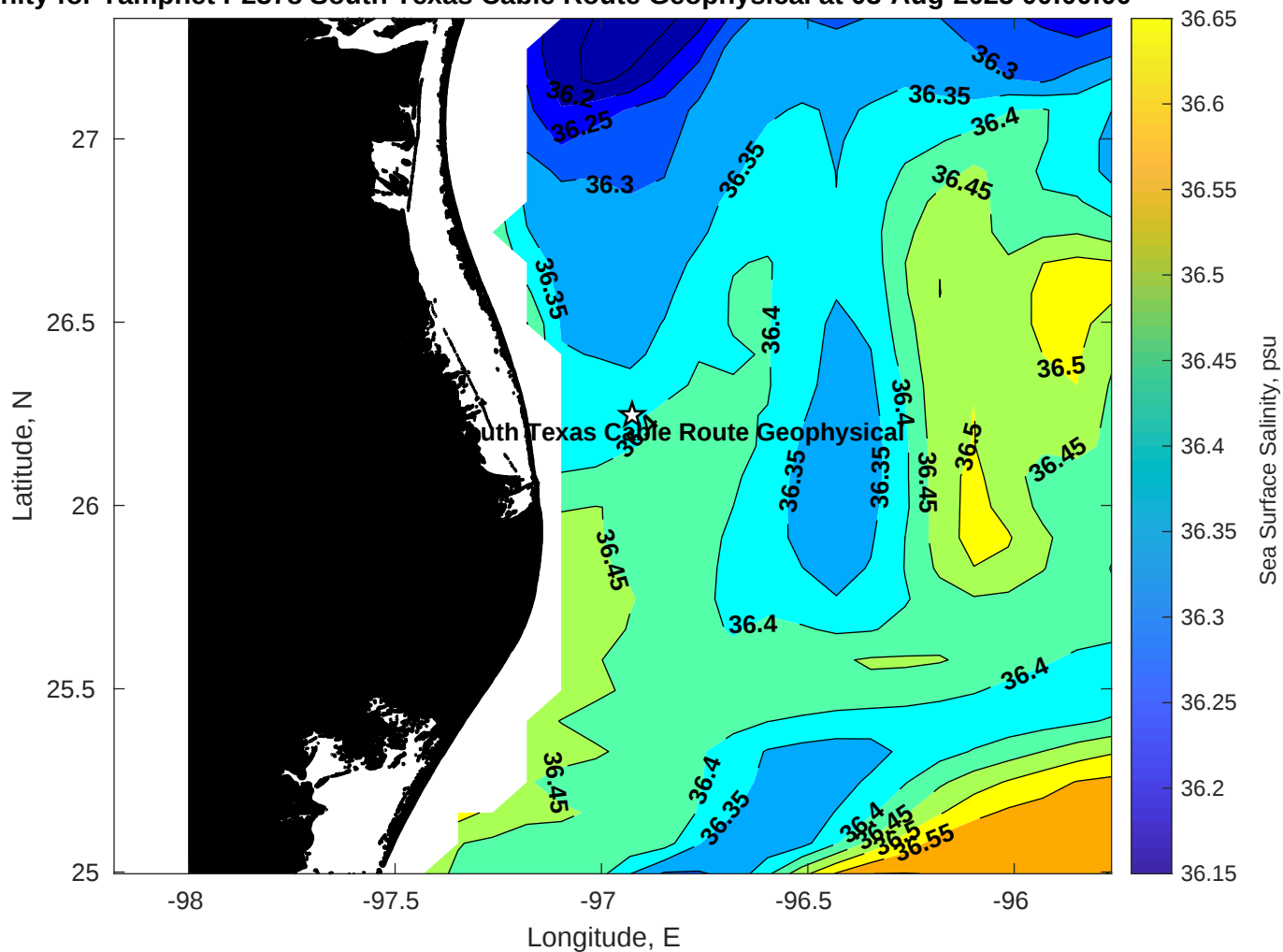
Surface Salinity for Tampnet P2378 South Texas Cable Route Geophysical at 03-Aug-2025 00:00:00
