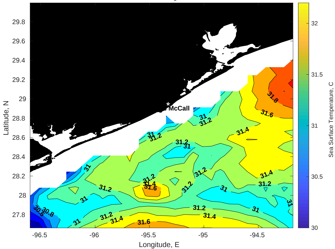
SST for Brooks McCall at 04-Aug-2025 00:00:00
