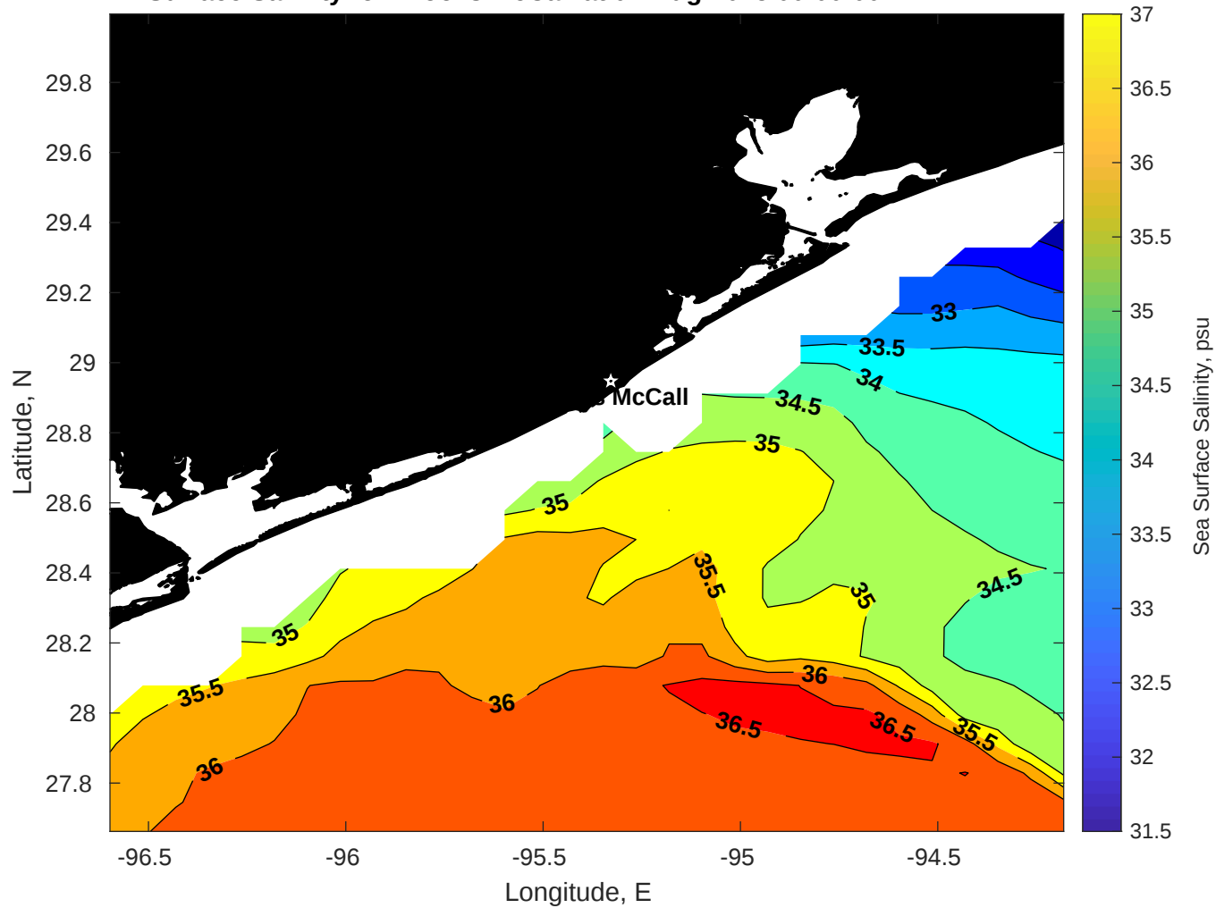
Surface Salinity for Brooks McCall at 04-Aug-2025 00:00:00
