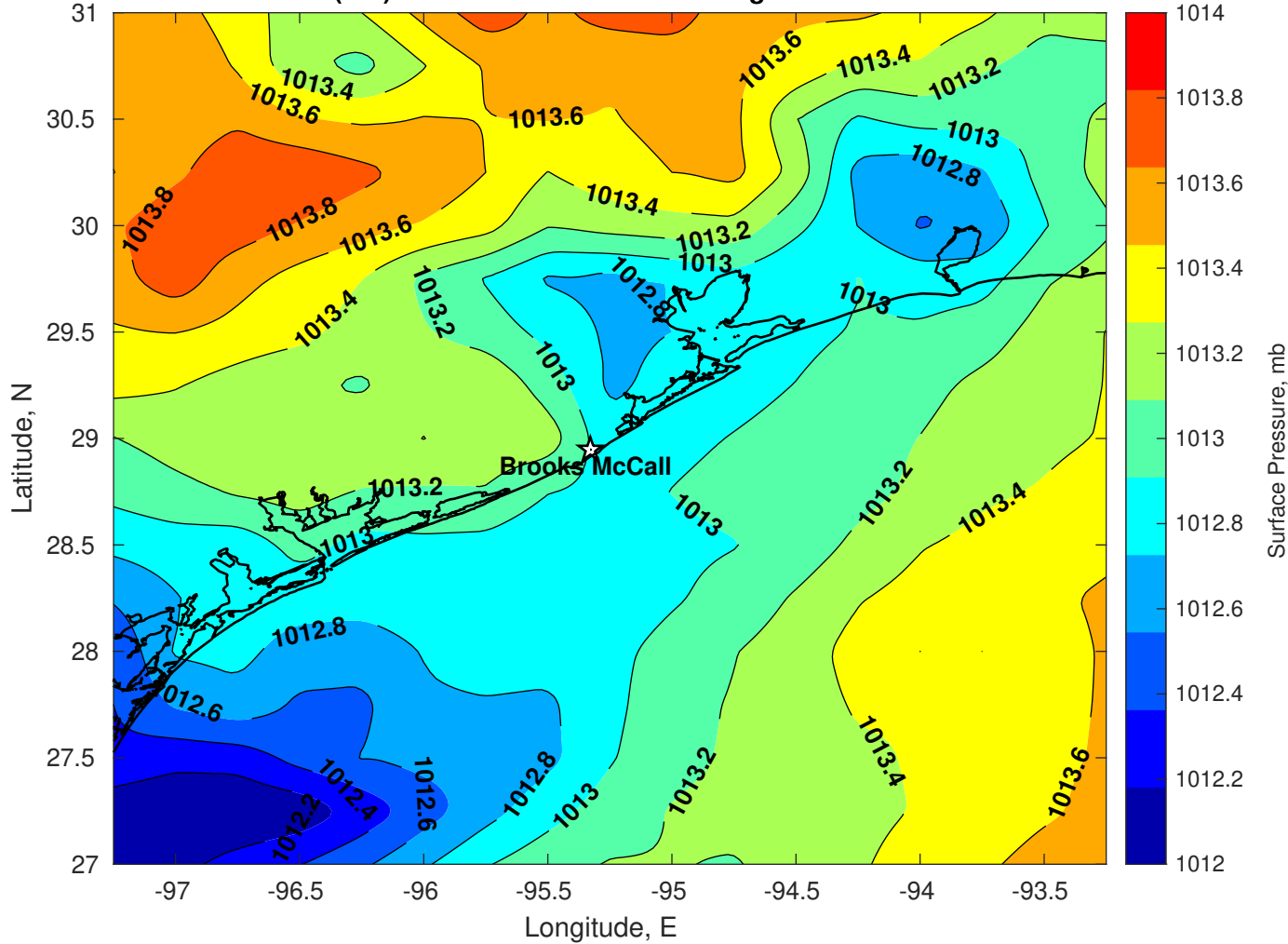
Surface Pressure (mb) for Brooks McCall at 05-Aug-2025 00:00:00
