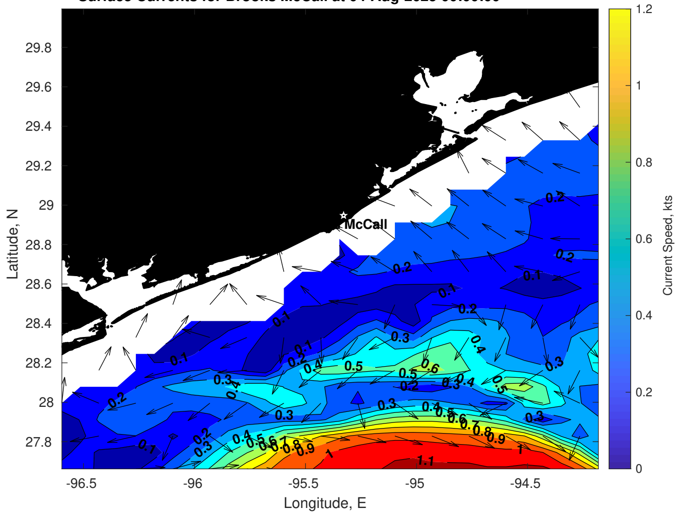
Surface Currents for Brooks McCall at 04-Aug-2025 00:00:00
