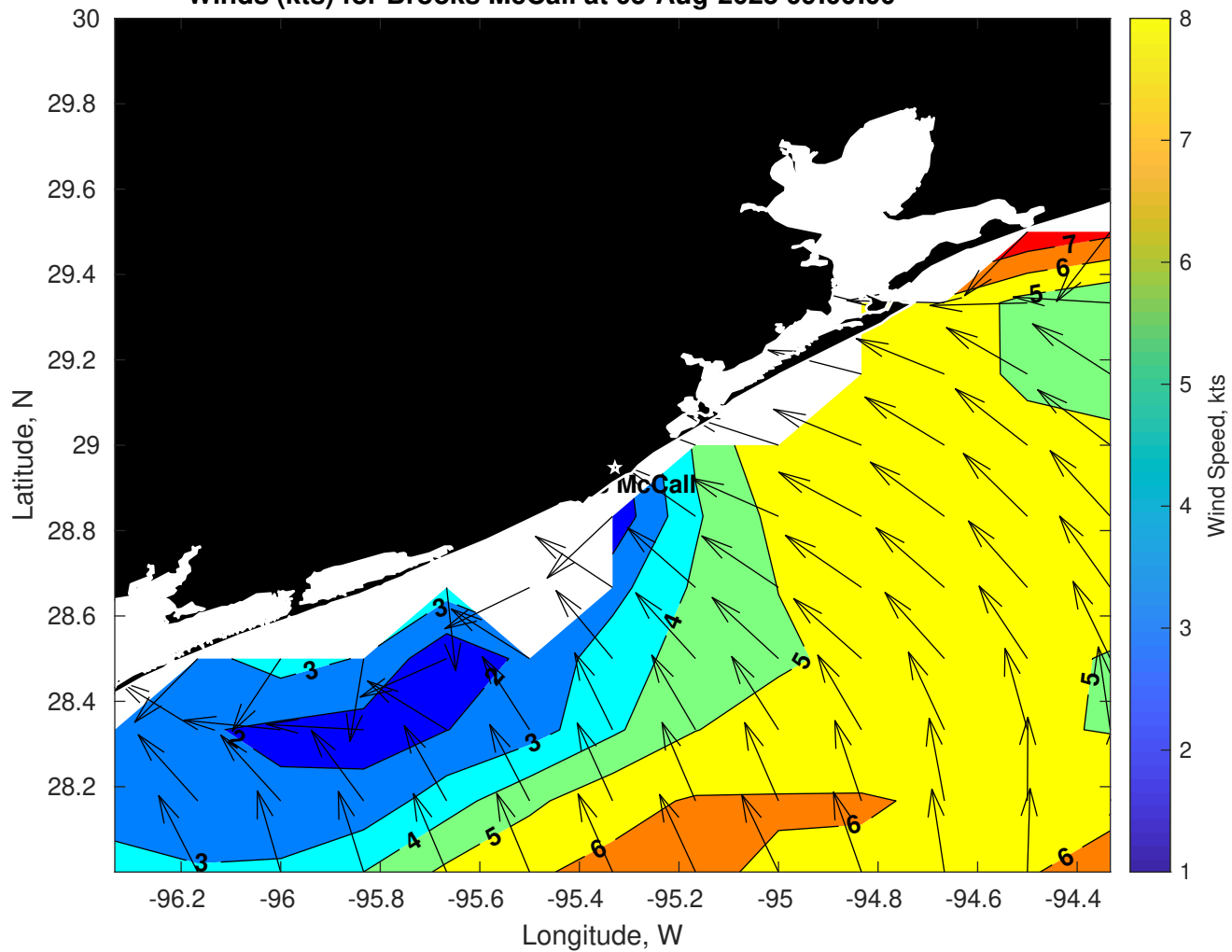
Winds (kts) for Brooks McCall at 05-Aug-2025 09:00:00
