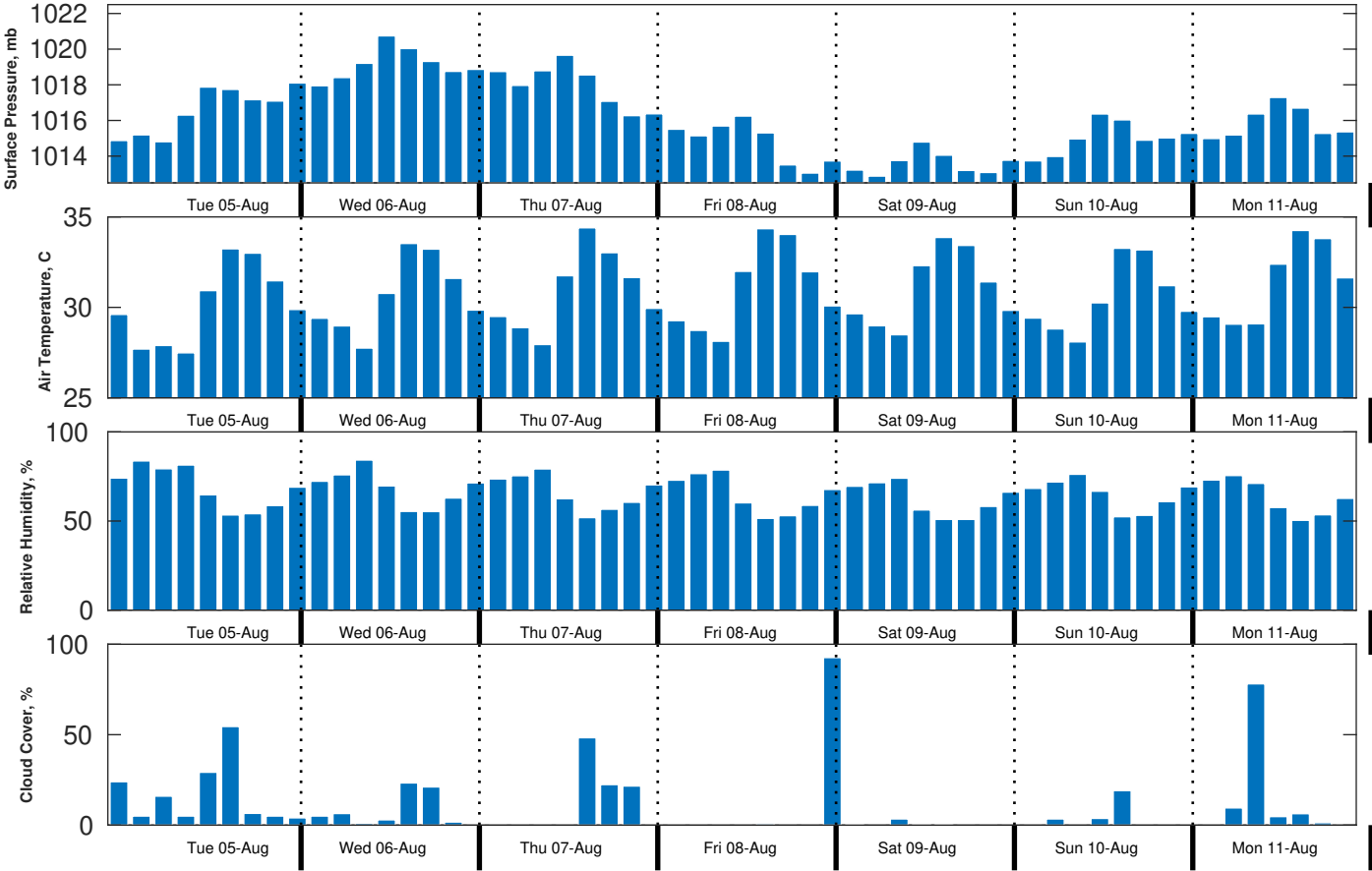
Met Forecast for Brooks McCall from 05-Aug-2025 00:00:00 to 12-Aug-2025 00:00:00
