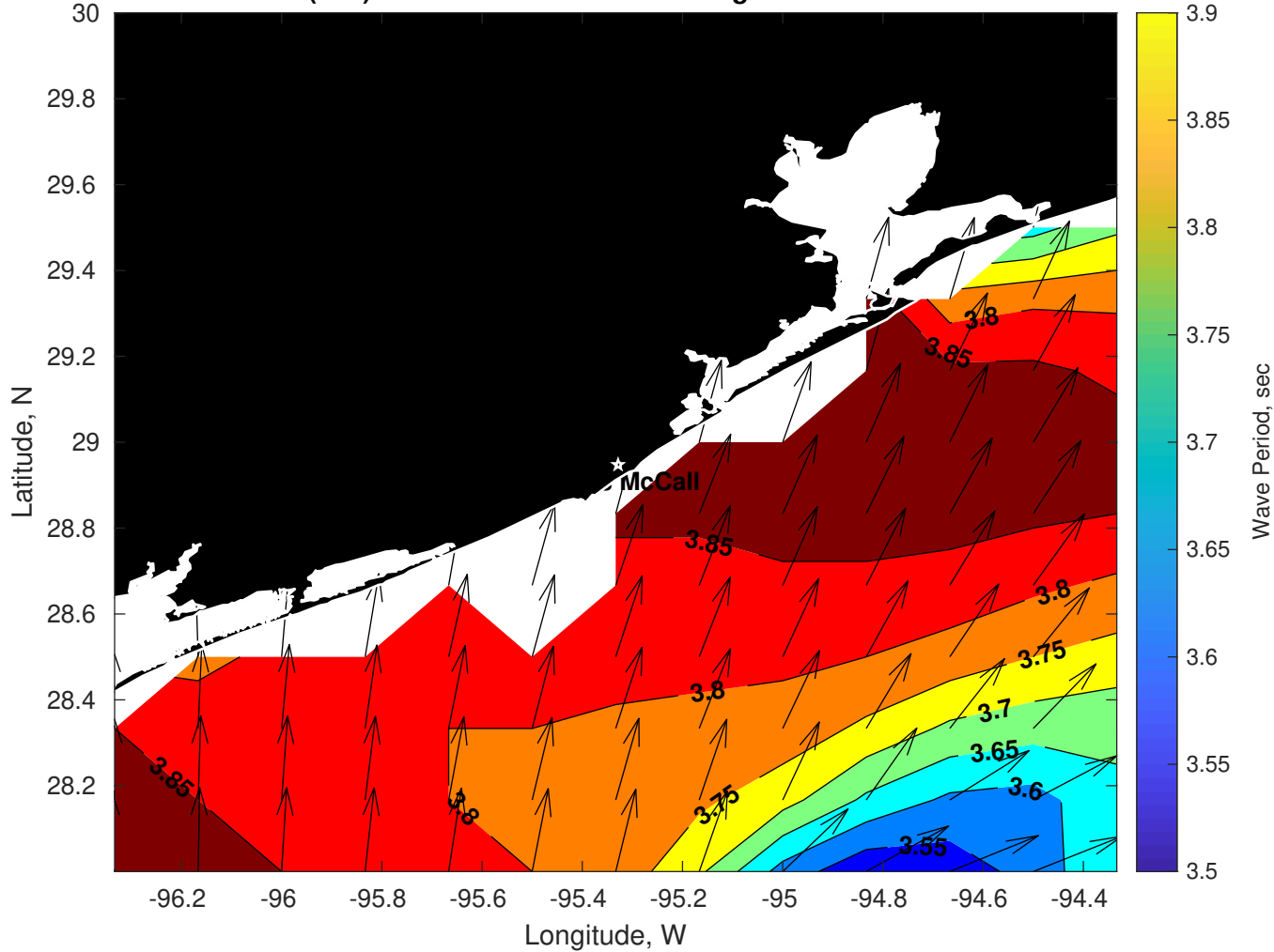
Wave Period (sec) for Brooks McCall at 05-Aug-2025 09:00:00
