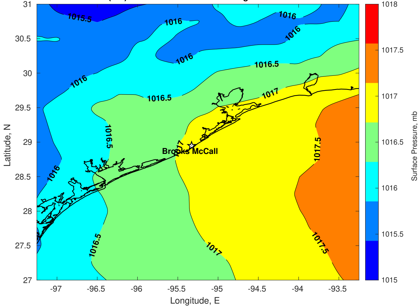
Surface Pressure (mb) for Brooks McCall at 06-Aug-2025 00:00:00
