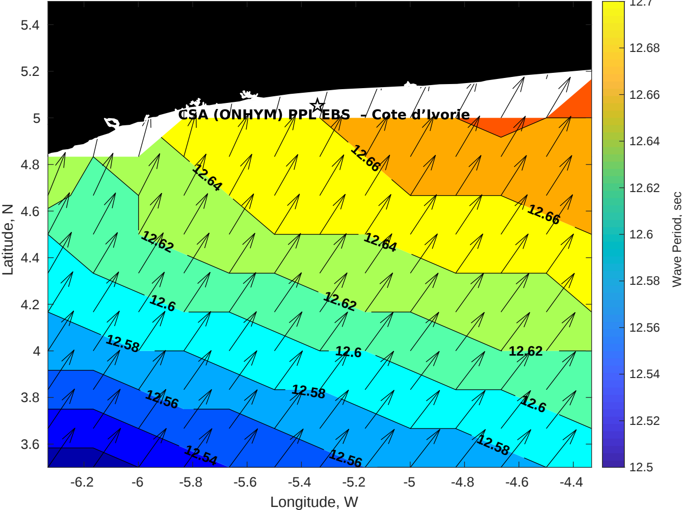
Wave Period (sec) for CSA (ONHYM) PPL EBS - Cote d'Ivoire at 05-Aug-2025 09:00:00
