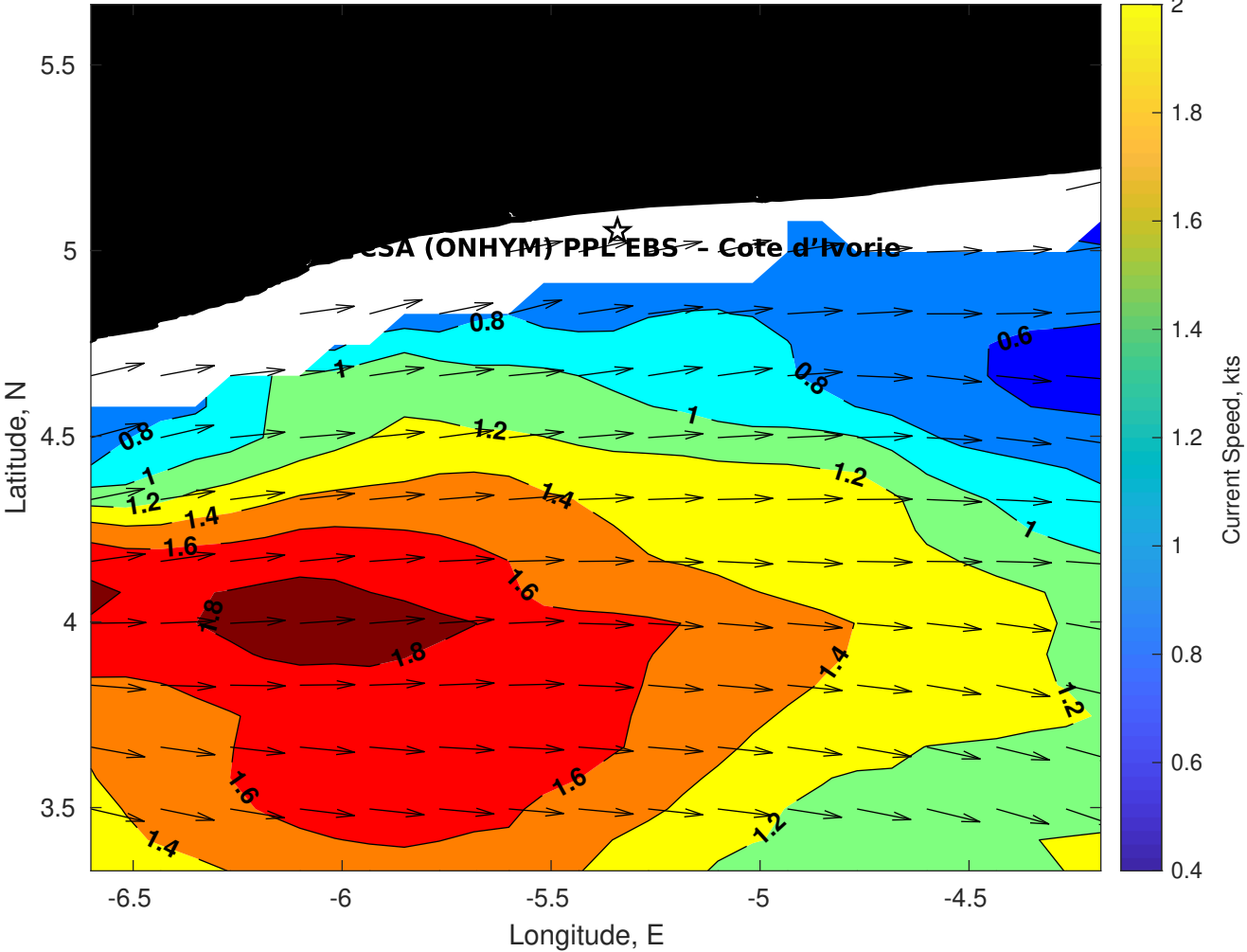
Surface Currents for CSA (ONHYM) PPL EBS - Cote d'Ivoire at 04-Aug-2025 00:00:00
