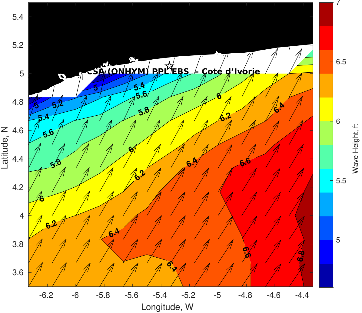
Wave Height (ft) for CSA (ONHYM) PPL EBS - Cote d'Ivoire at 05-Aug-2025 09:00:00
