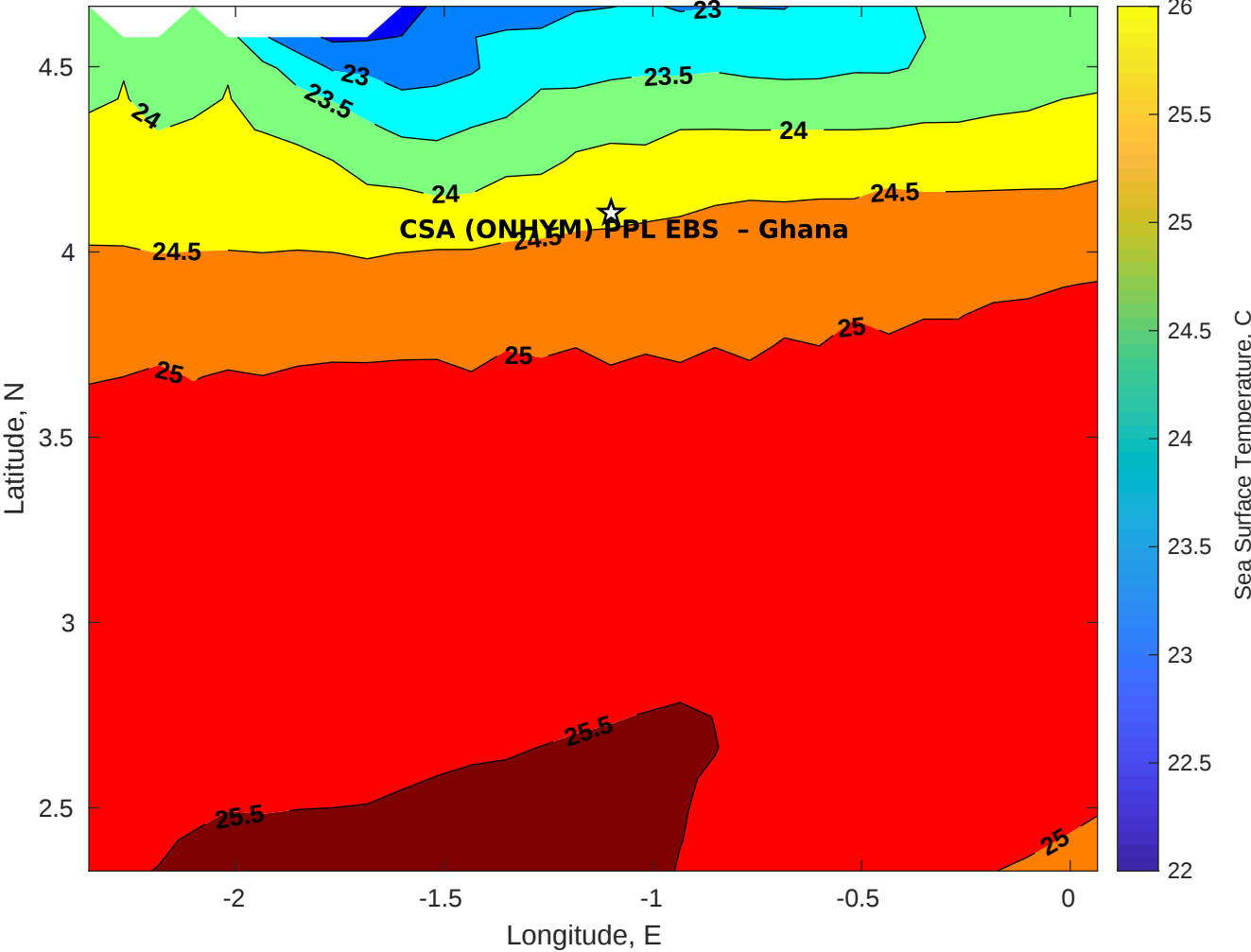
SST for CSA (ONHYM) PPL EBS - Ghana at 04-Aug-2025 00:00:00
