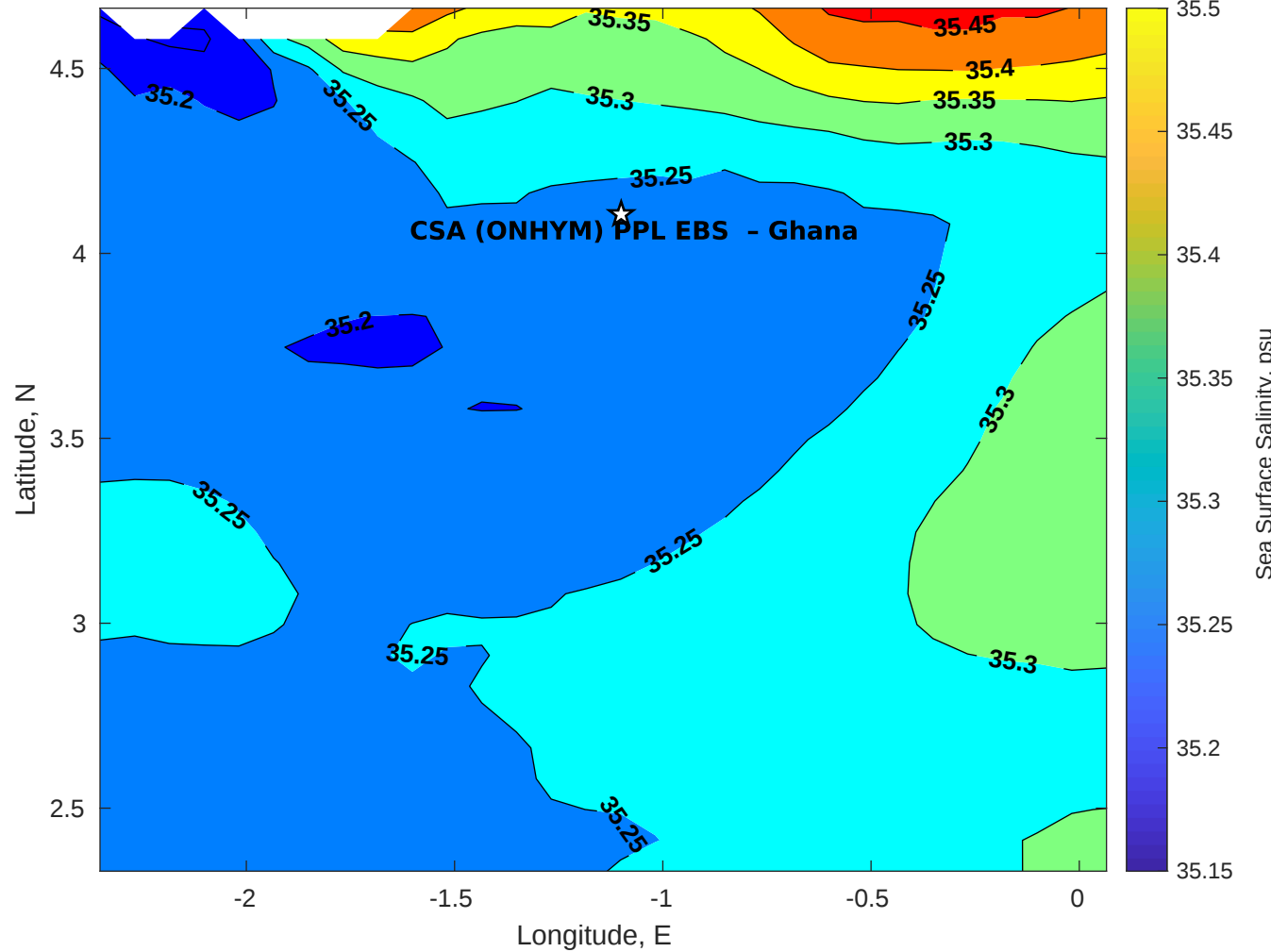
Surface Salinity for CSA (ONHYM) PPL EBS - Ghana at 04-Aug-2025 00:00:00
