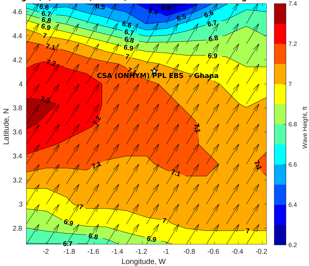
Wave Height (ft) for CSA (ONHYM) PPL EBS - Ghana at 05-Aug-2025 09:00:00
