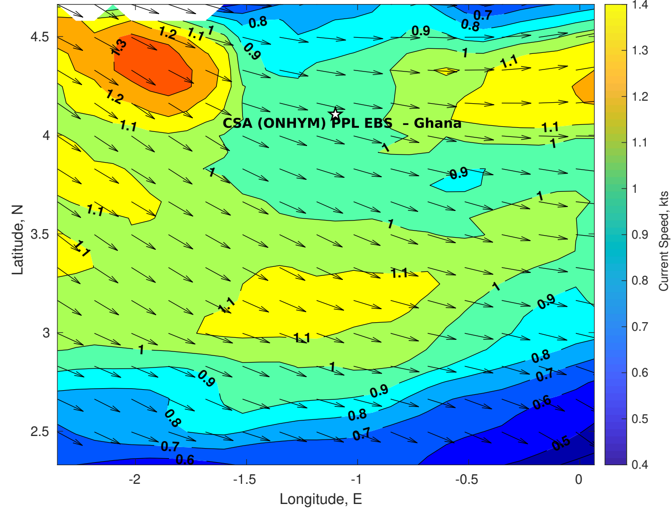
Surface Currents for CSA (ONHYM) PPL EBS - Ghana at 04-Aug-2025 00:00:00
