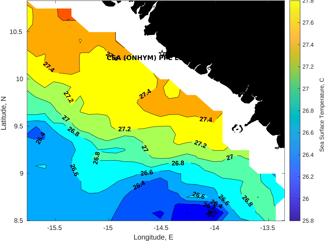
SST for CSA (ONHYM) PPL EBS - Guinea at 04-Aug-2025 00:00:00
