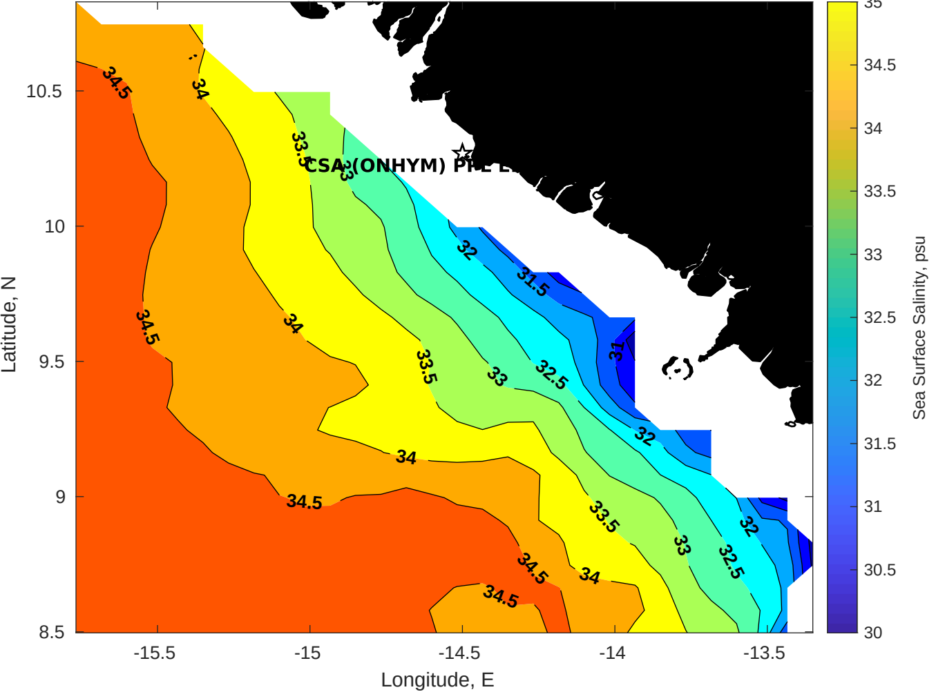
Surface Salinity for CSA (ONHYM) PPL EBS - Guinea at 04-Aug-2025 00:00:00
