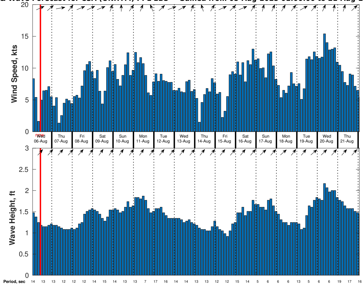
Wind & Wave Forecast for CSA (ONHYM) PPL EBS - Guinea from 05-Aug-2025 01:00:00 to 21-Aug-2025 01:00:00
