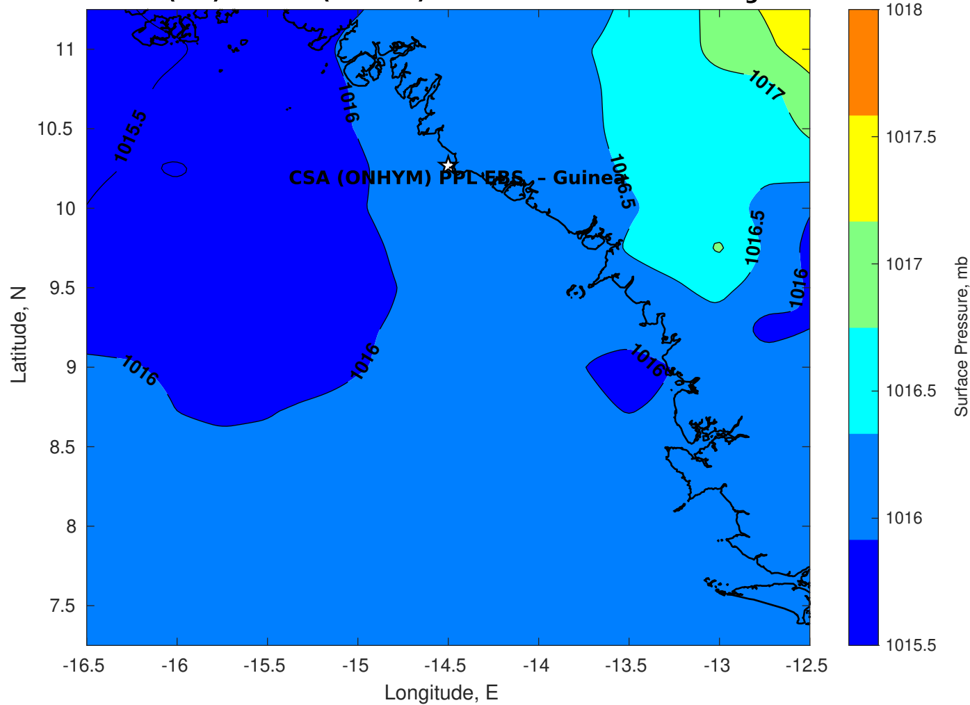
Surface Pressure (mb) for CSA (ONHYM) PPL EBS - Guinea at 06-Aug-2025 00:00:00
