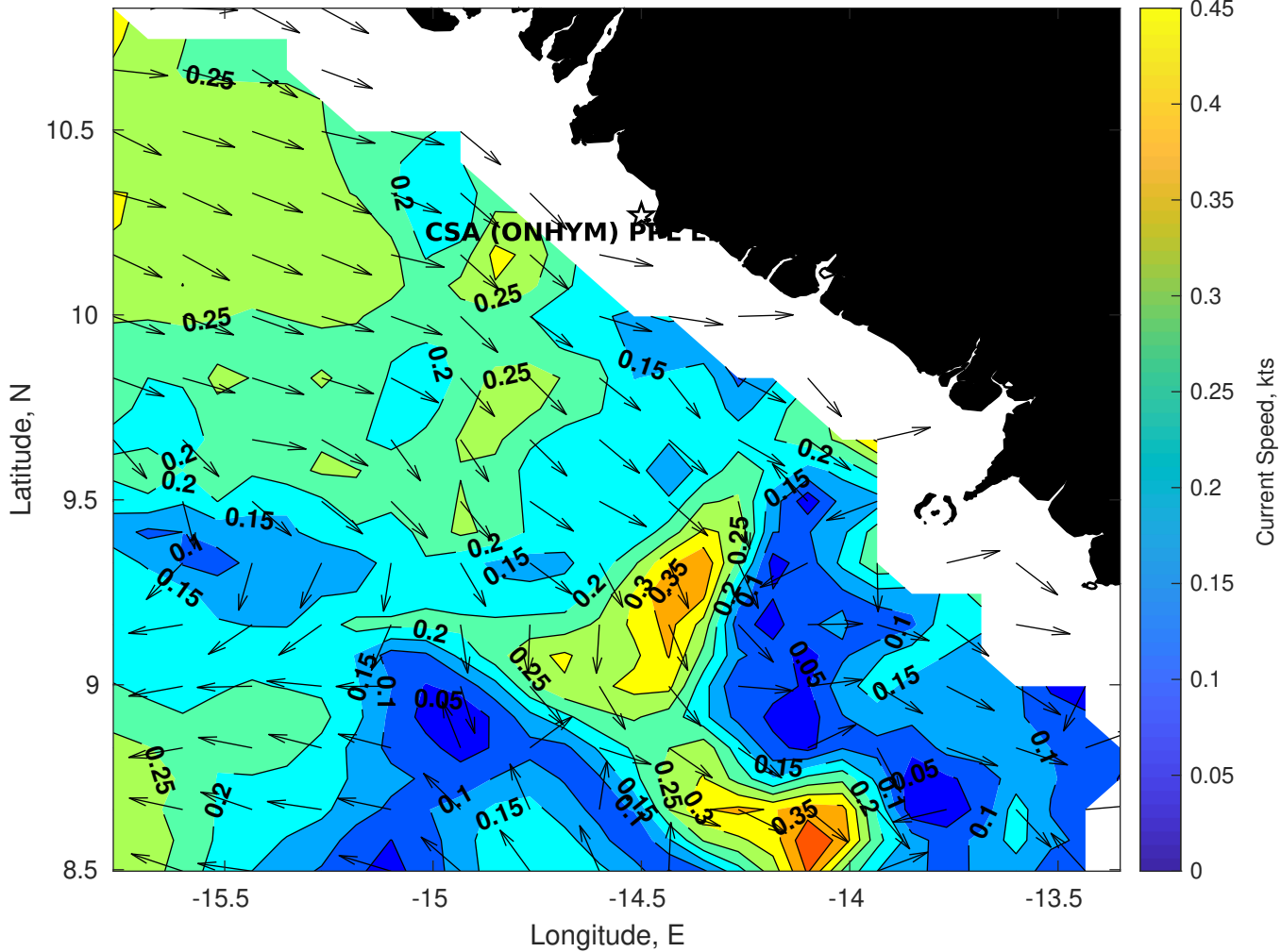
Surface Currents for CSA (ONHYM) PPL EBS - Guinea at 04-Aug-2025 00:00:00
