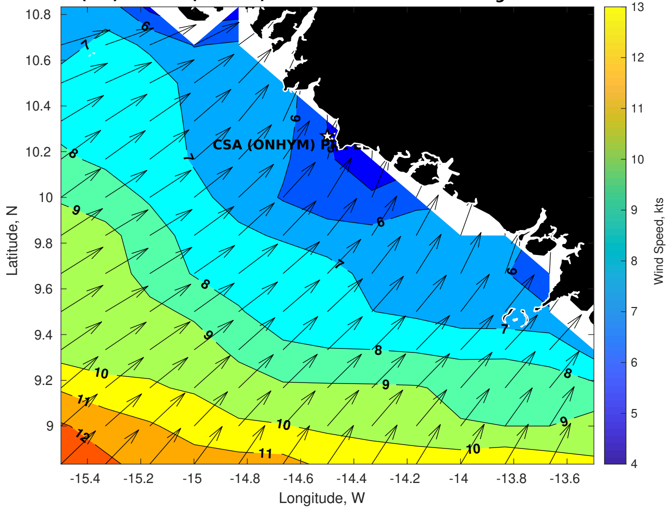
Winds (kts) for CSA (ONHYM) PPL EBS - Guinea at 05-Aug-2025 09:00:00
