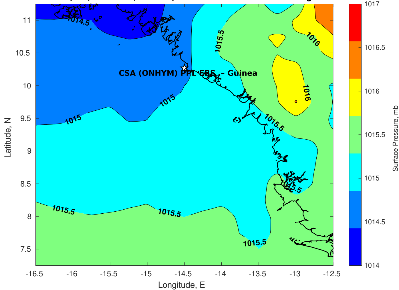
Surface Pressure (mb) for CSA (ONHYM) PPL EBS - Guinea at 05-Aug-2025 00:00:00
