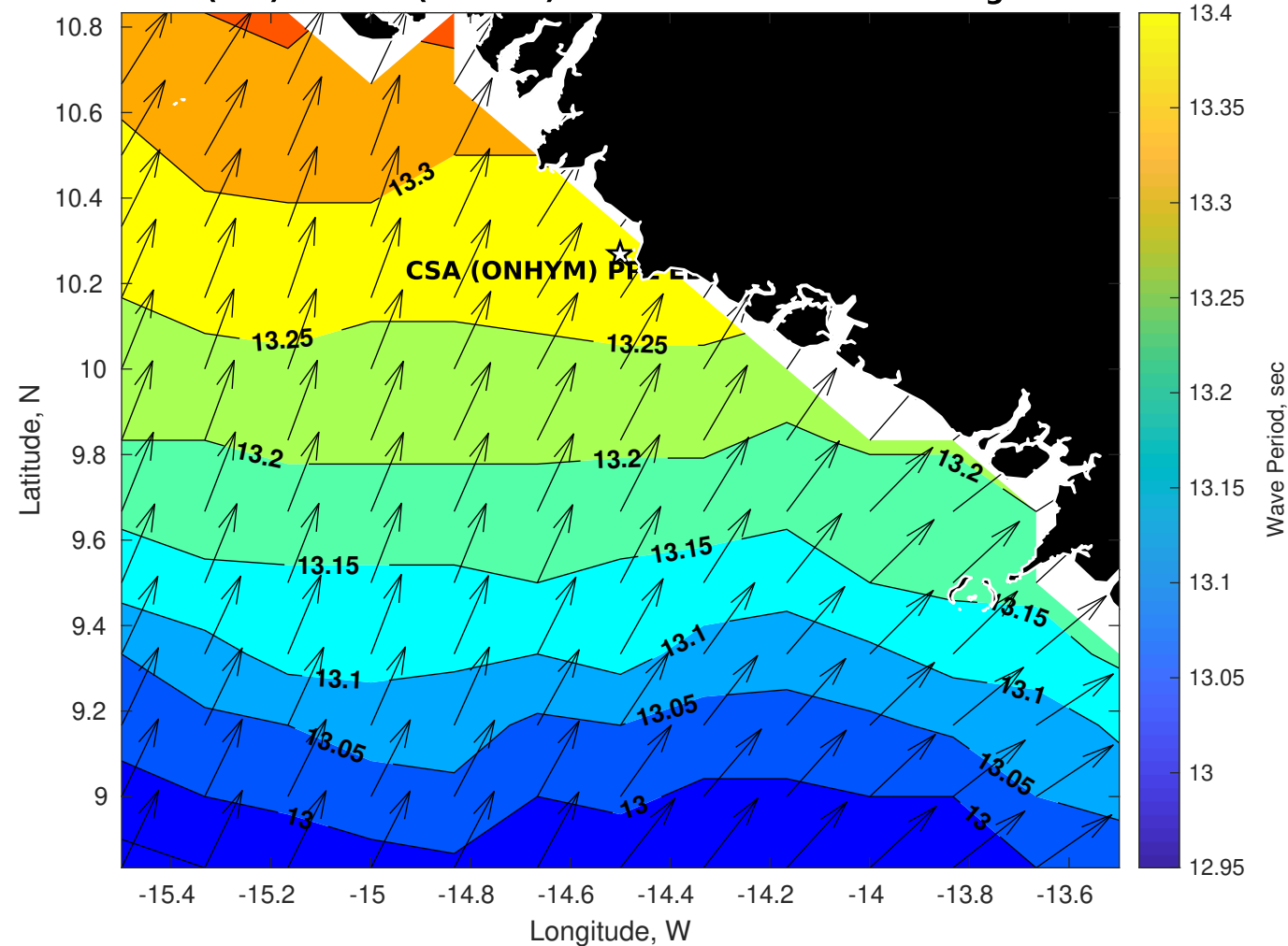
Wave Period (sec) for CSA (ONHYM) PPL EBS - Guinea at 05-Aug-2025 09:00:00
