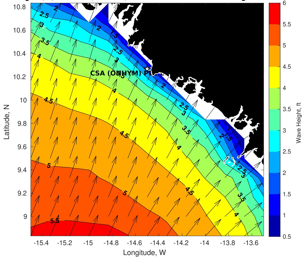
Wave Height (ft) for CSA (ONHYM) PPL EBS - Guinea at 05-Aug-2025 09:00:00
