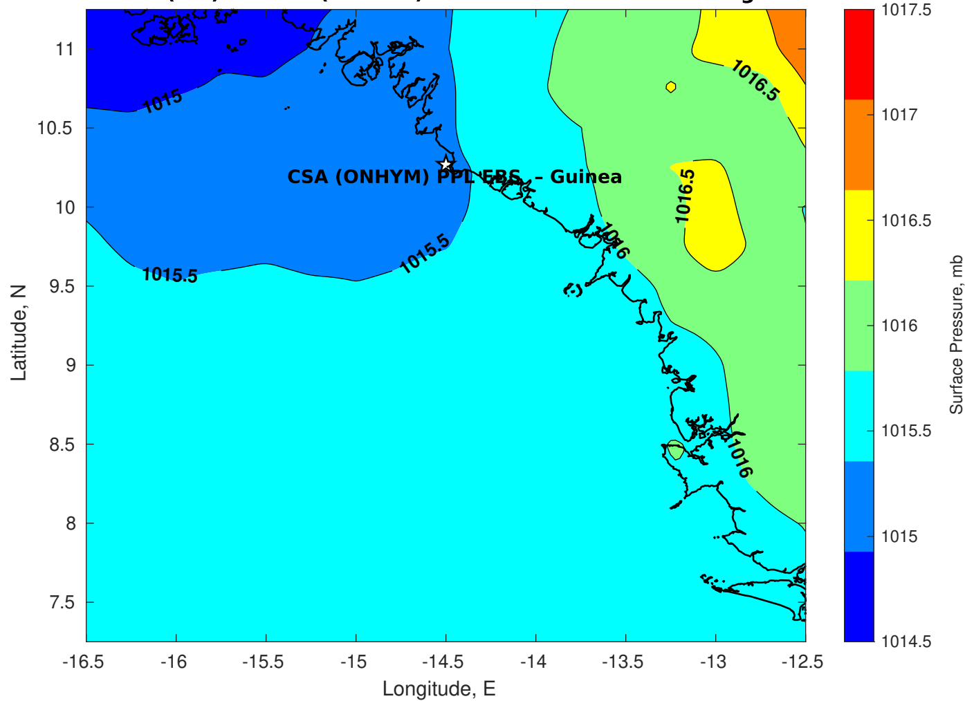
Surface Pressure (mb) for CSA (ONHYM) PPL EBS - Guinea at 07-Aug-2025 00:00:00
