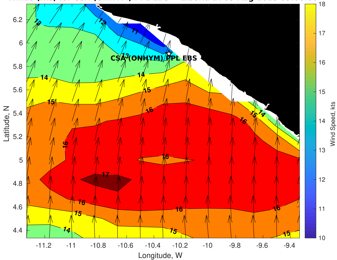
Winds (kts) for CSA (ONHYM) PPL EBS - Liberia at 05-Aug-2025 09:00:00
