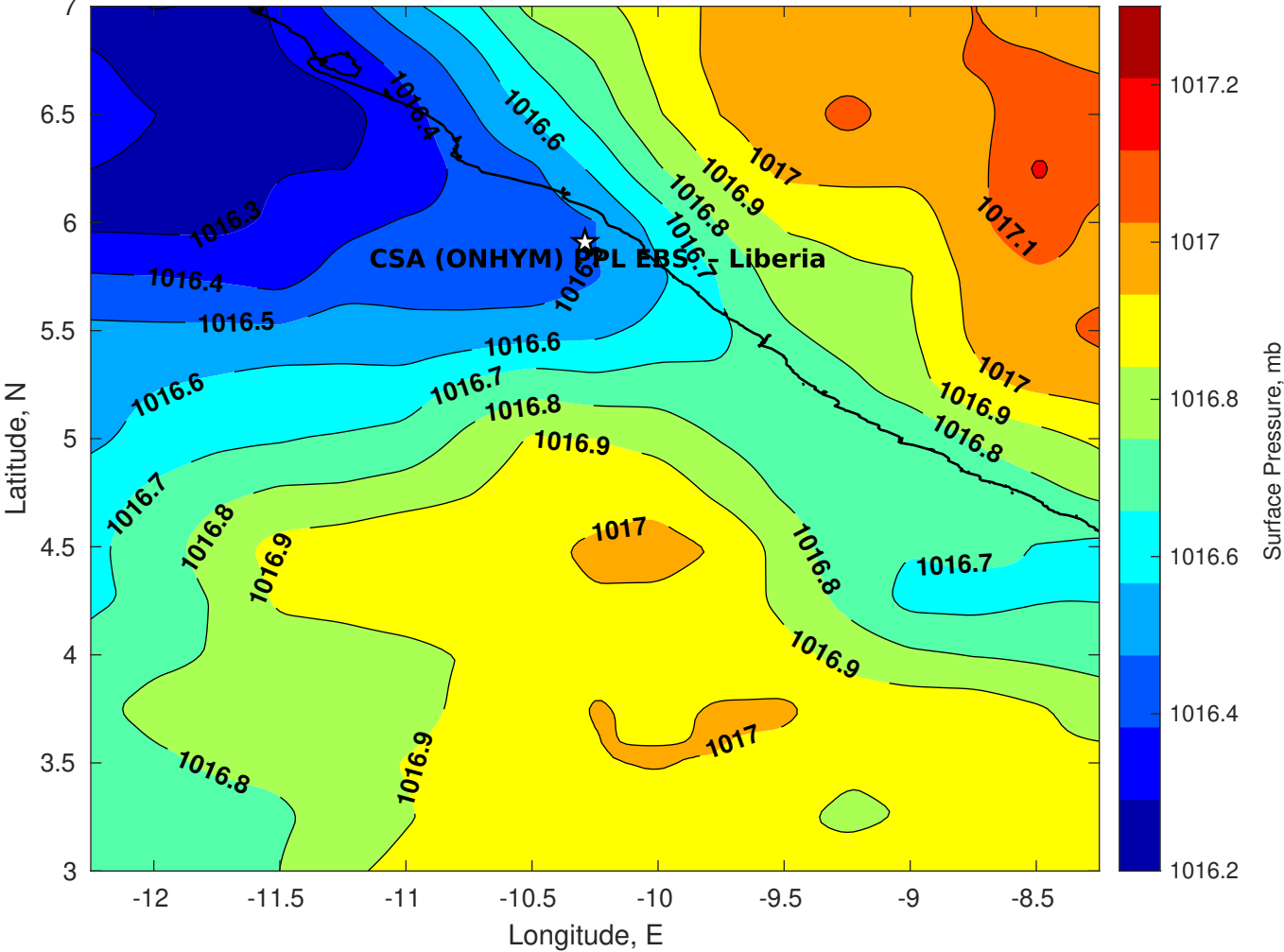
Surface Pressure (mb) for CSA (ONHYM) PPL EBS - Liberia at 06-Aug-2025 00:00:00
