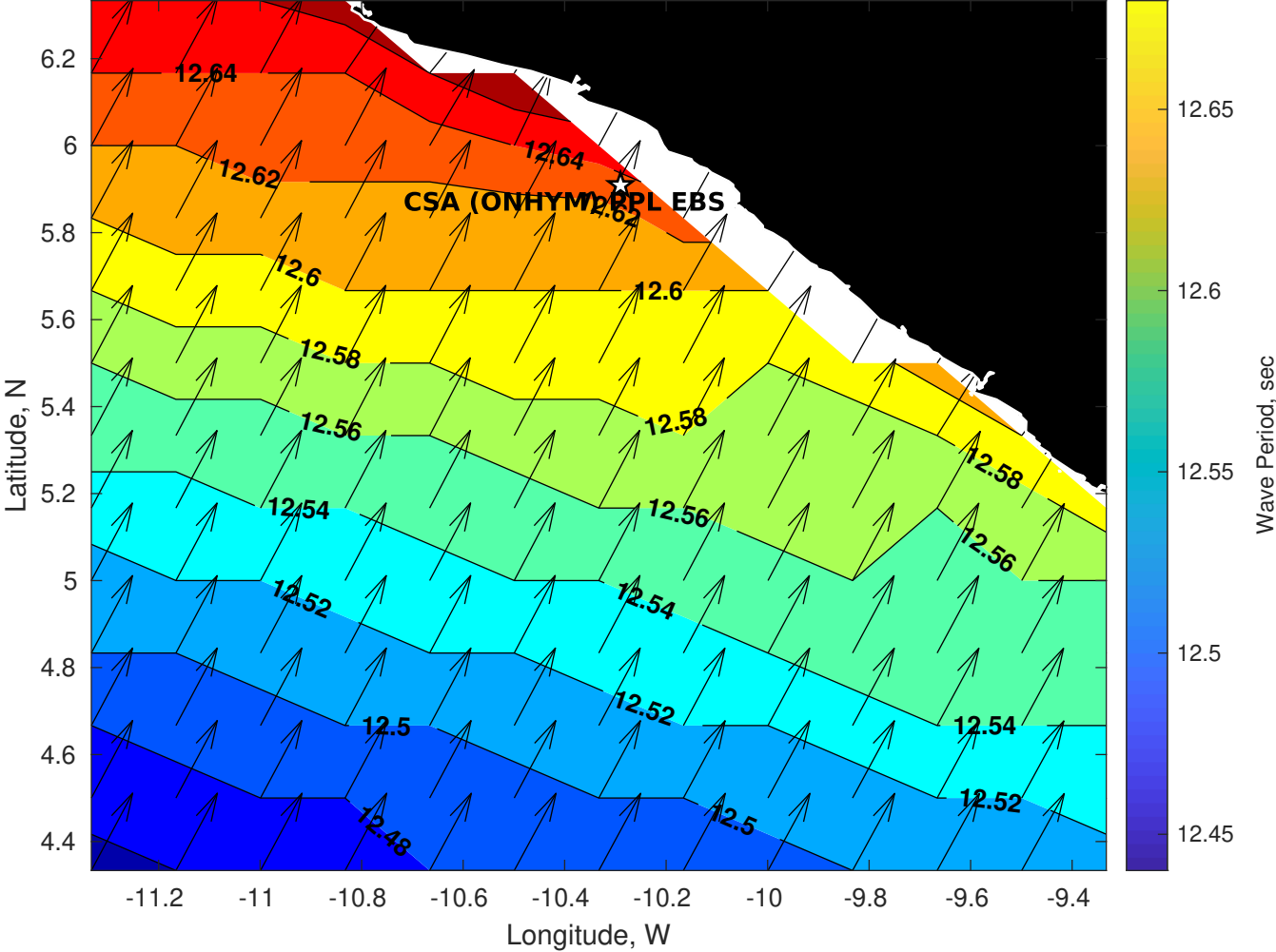
Wave Period (sec) for CSA (ONHYM) PPL EBS - Liberia at 05-Aug-2025 09:00:00
