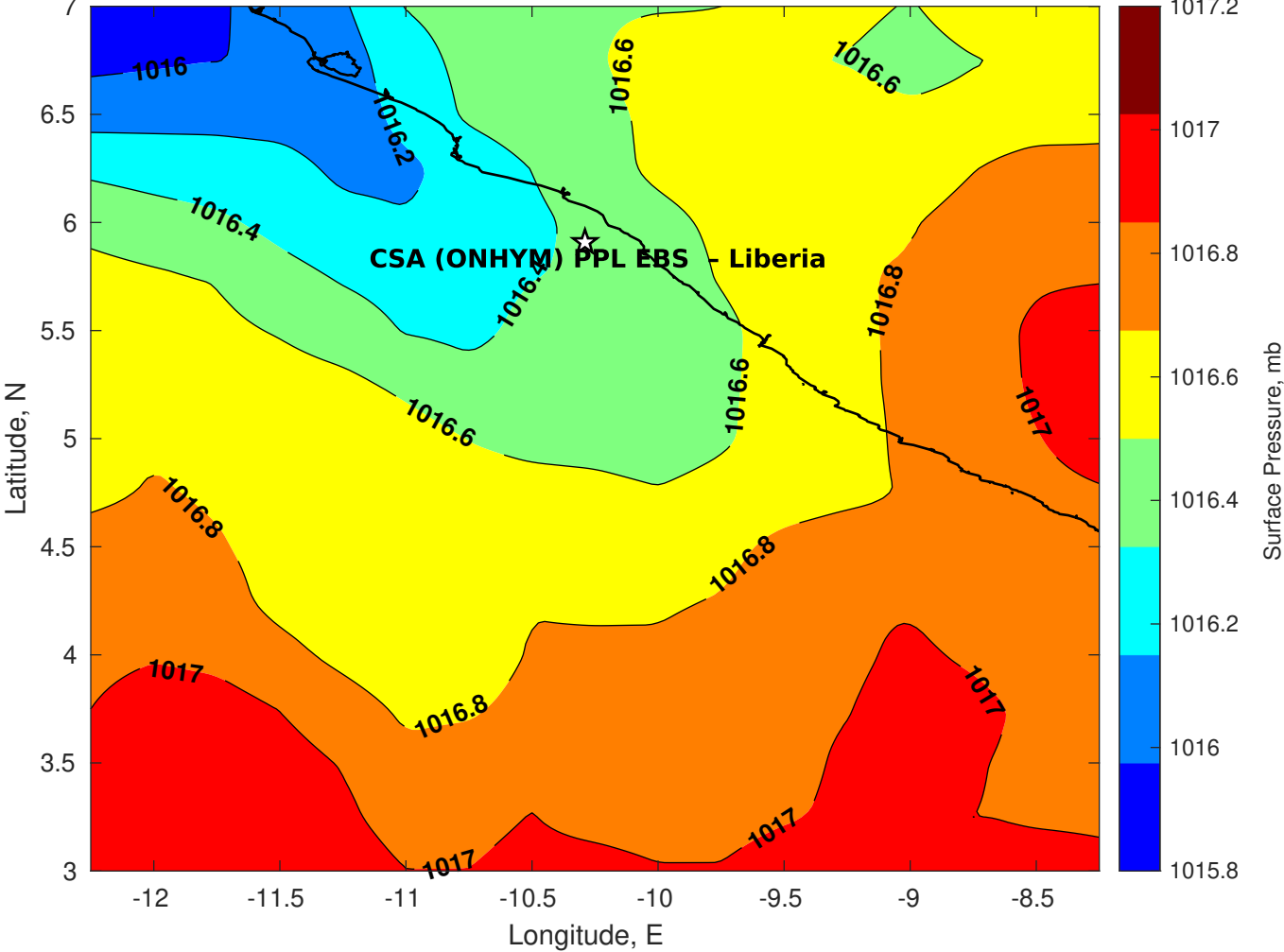
Surface Pressure (mb) for CSA (ONHYM) PPL EBS - Liberia at 05-Aug-2025 00:00:00
