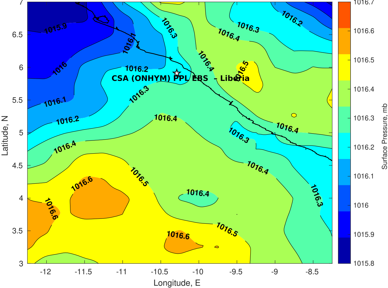
Surface Pressure (mb) for CSA (ONHYM) PPL EBS - Liberia at 07-Aug-2025 00:00:00
