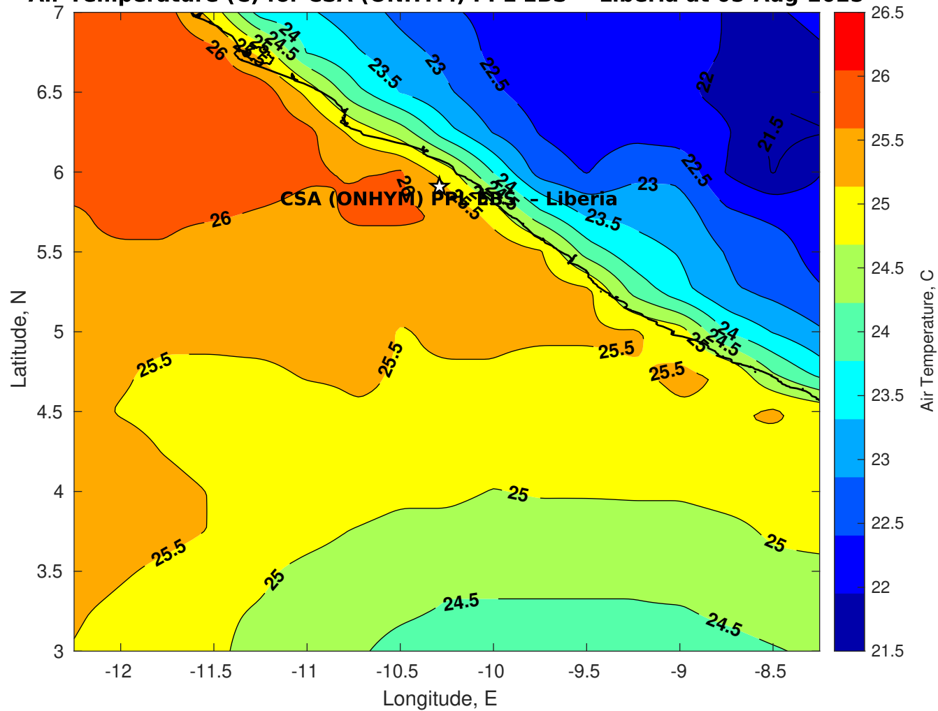
Air Temperature (C) for CSA (ONHYM) PPL EBS - Liberia at 05-Aug-2025
