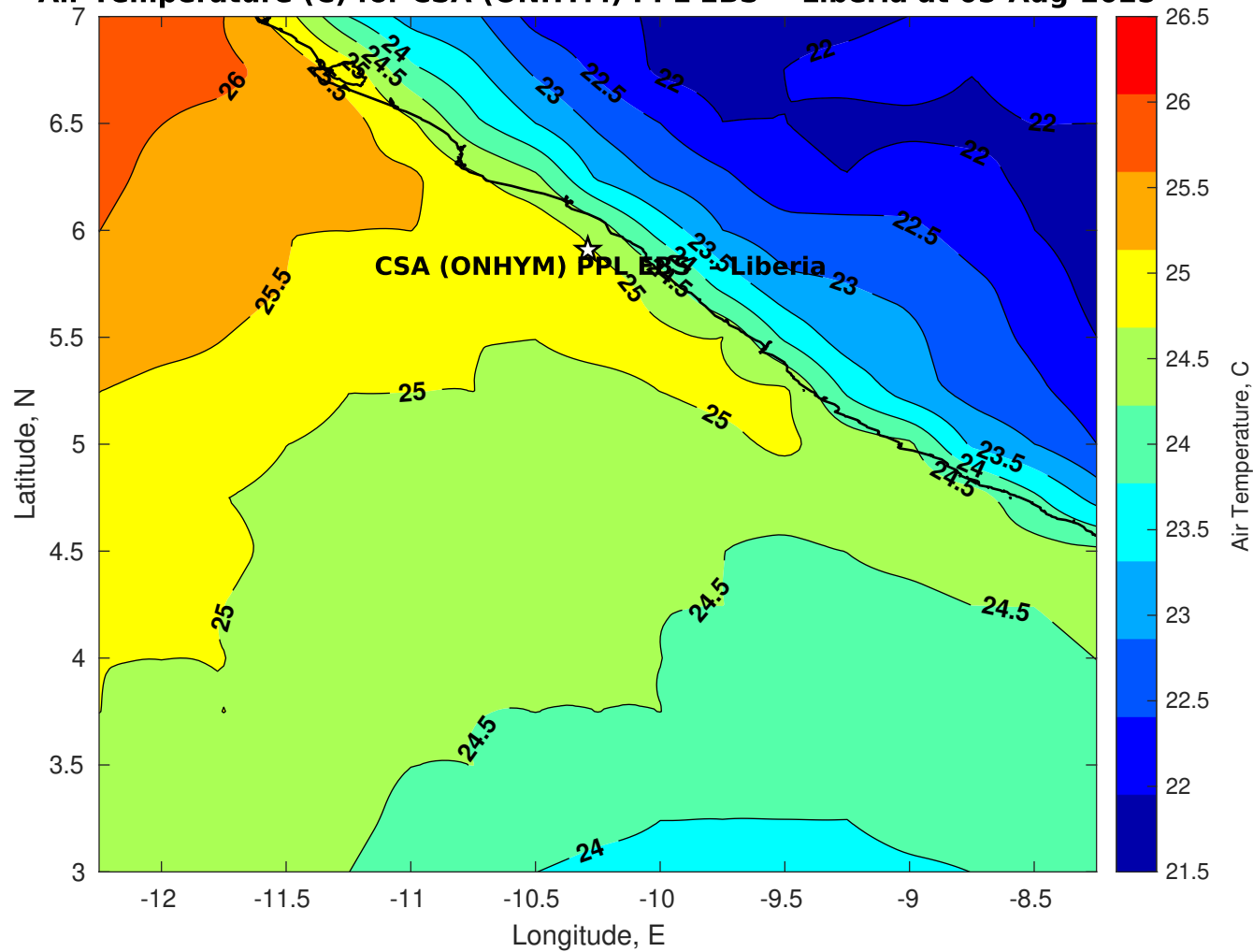
Air Temperature (C) for CSA (ONHYM) PPL EBS - Liberia at 05-Aug-2025
