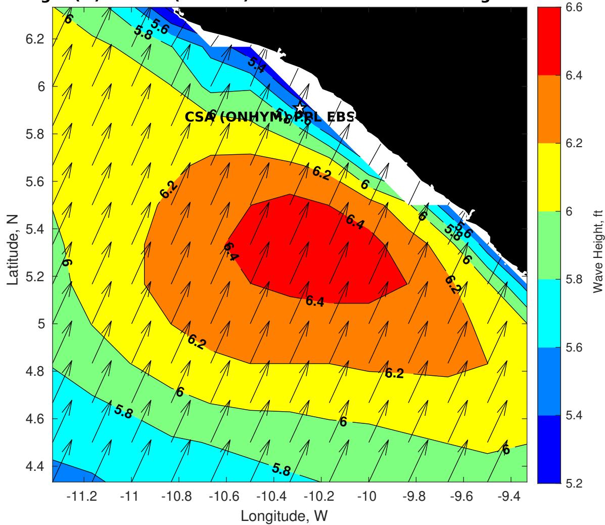
Wave Height (ft) for CSA (ONHYM) PPL EBS - Liberia at 05-Aug-2025 09:00:00
