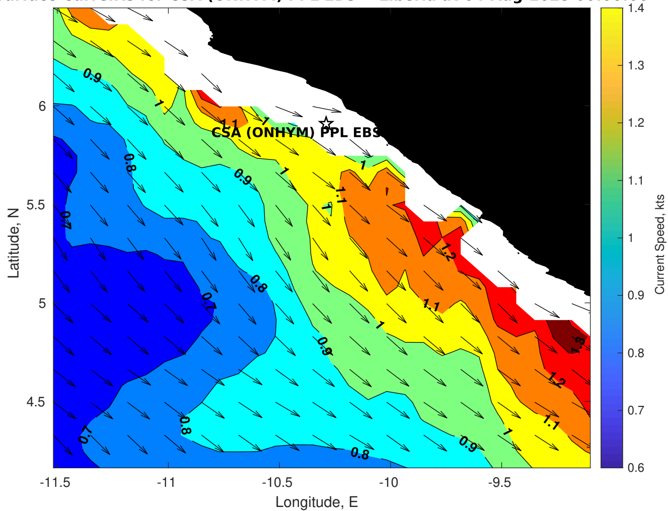
Surface Currents for CSA (ONHYM) PPL EBS - Liberia at 04-Aug-2025 00:00:00
