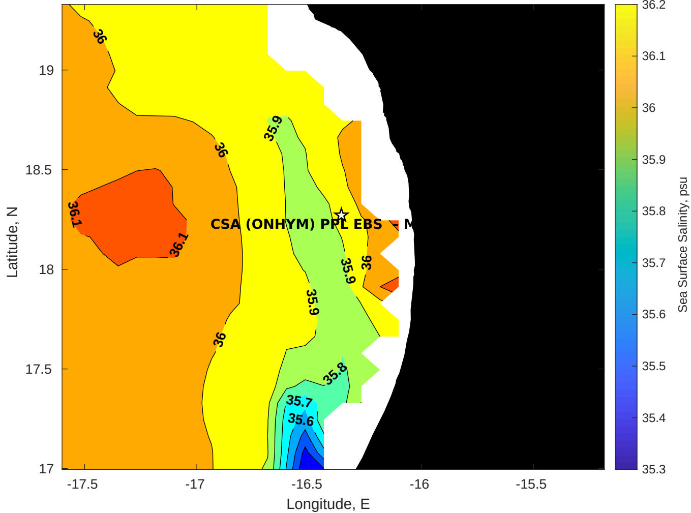
Surface Salinity for CSA (ONHYM) PPL EBS - Mauritania at 04-Aug-2025 00:00:00
