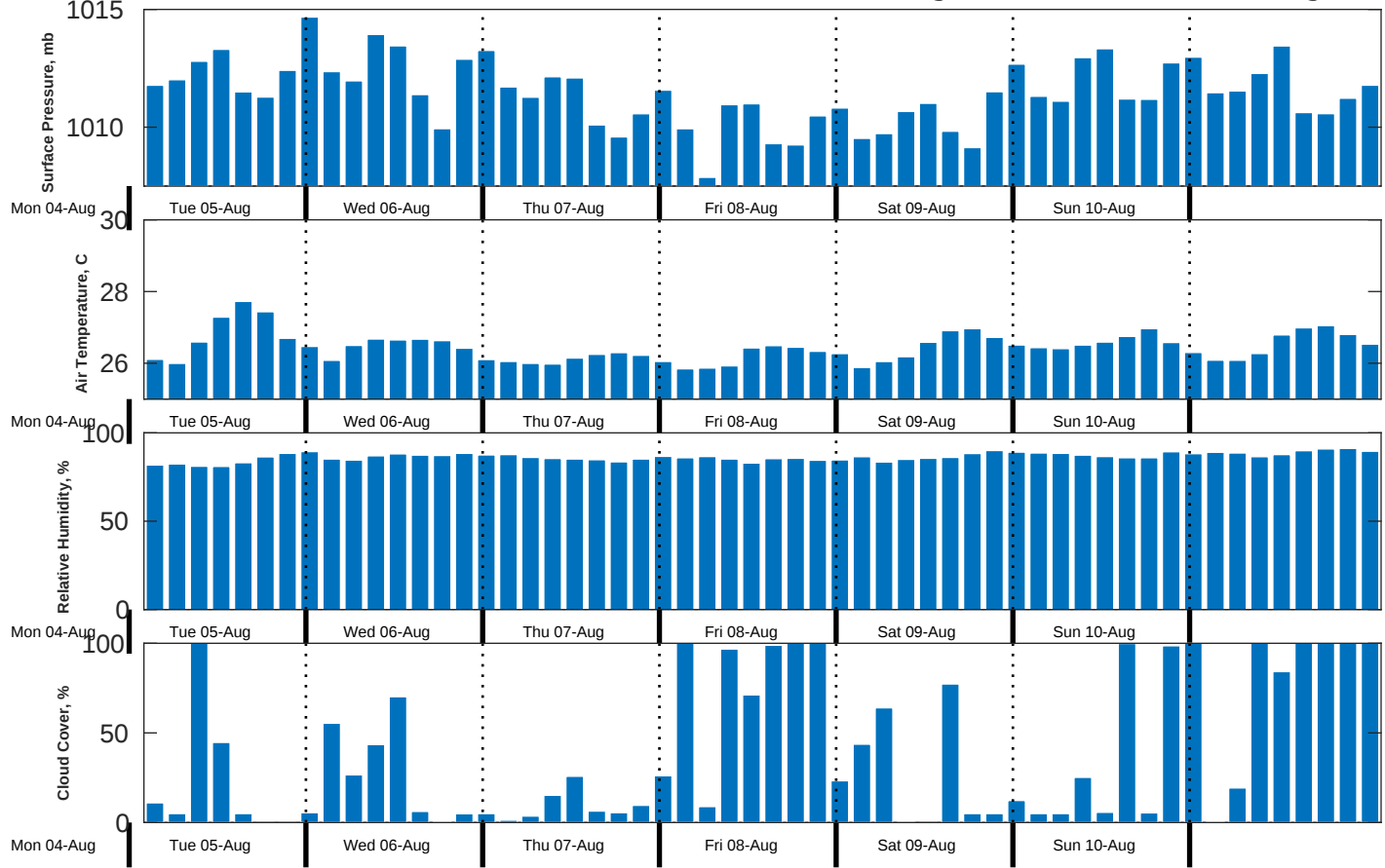
Met Forecast for CSA (ONHYM) PPL EBS - Mauritania from 05-Aug-2025 00:00:00 to 12-Aug-2025 00:00:00
