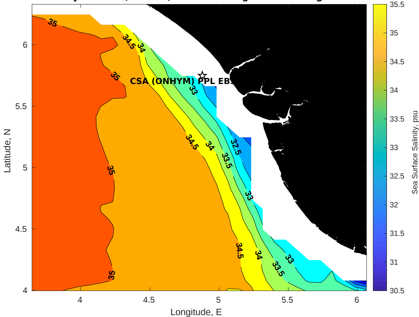
Surface Salinity for CSA (ONHYM) PPL EBS - Nigeria at 04-Aug-2025 00:00:00
