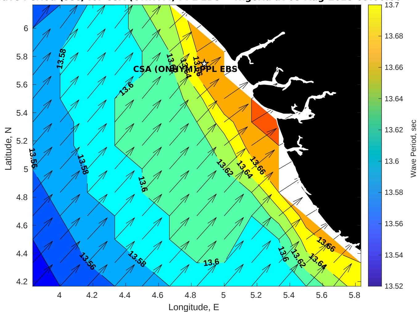
Wave Period (sec) for CSA (ONHYM) PPL EBS - Nigeria at 05-Aug-2025 09:00:00
