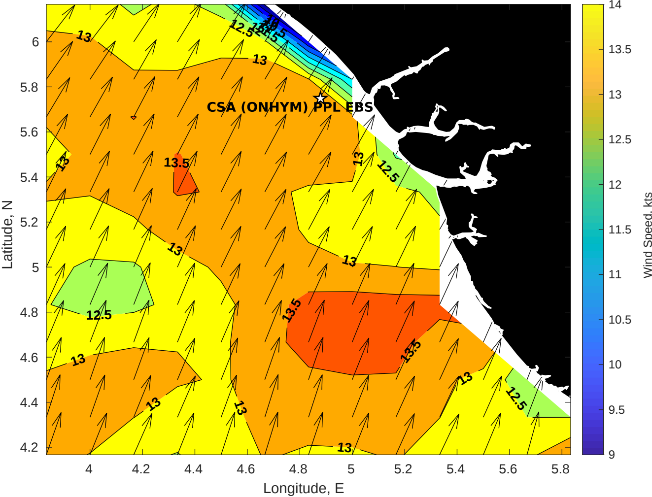
Winds (kts) for CSA (ONHYM) PPL EBS - Nigeria at 05-Aug-2025 09:00:00
