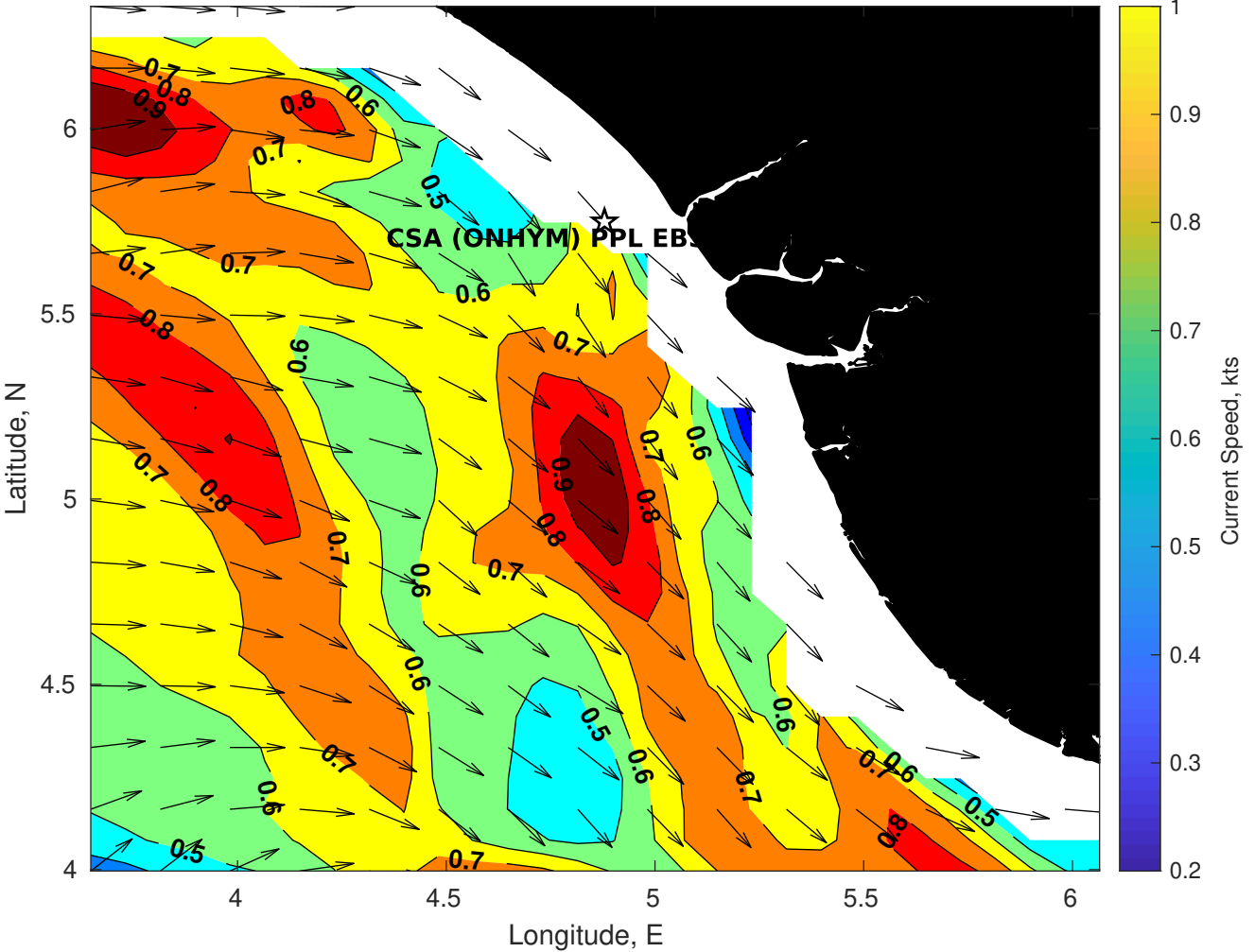
Surface Currents for CSA (ONHYM) PPL EBS - Nigeria at 04-Aug-2025 00:00:00
