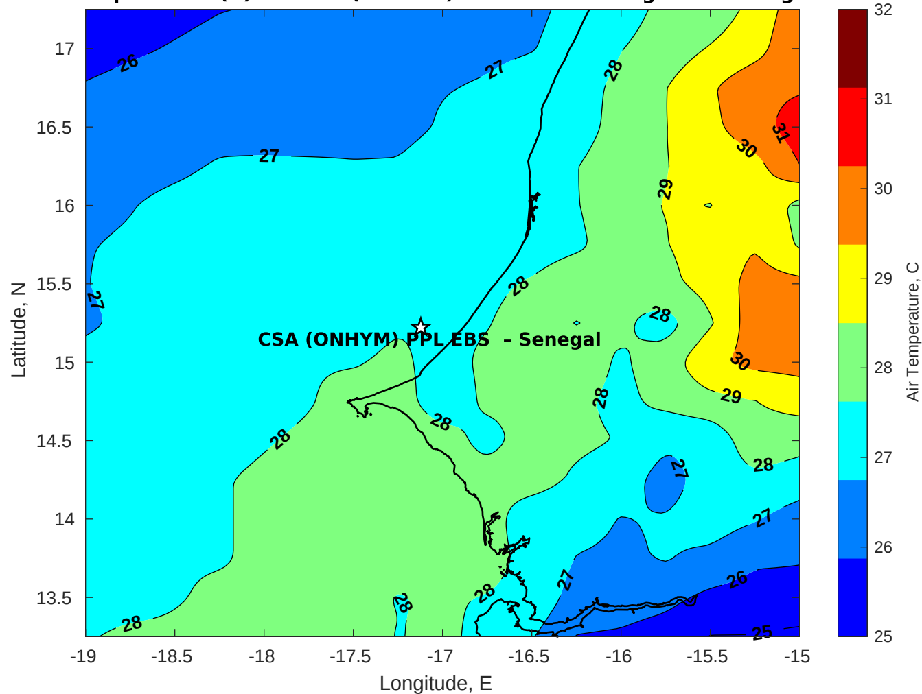
Air Temperature (C) for CSA (ONHYM) PPL EBS - Senegal at 05-Aug-2025
