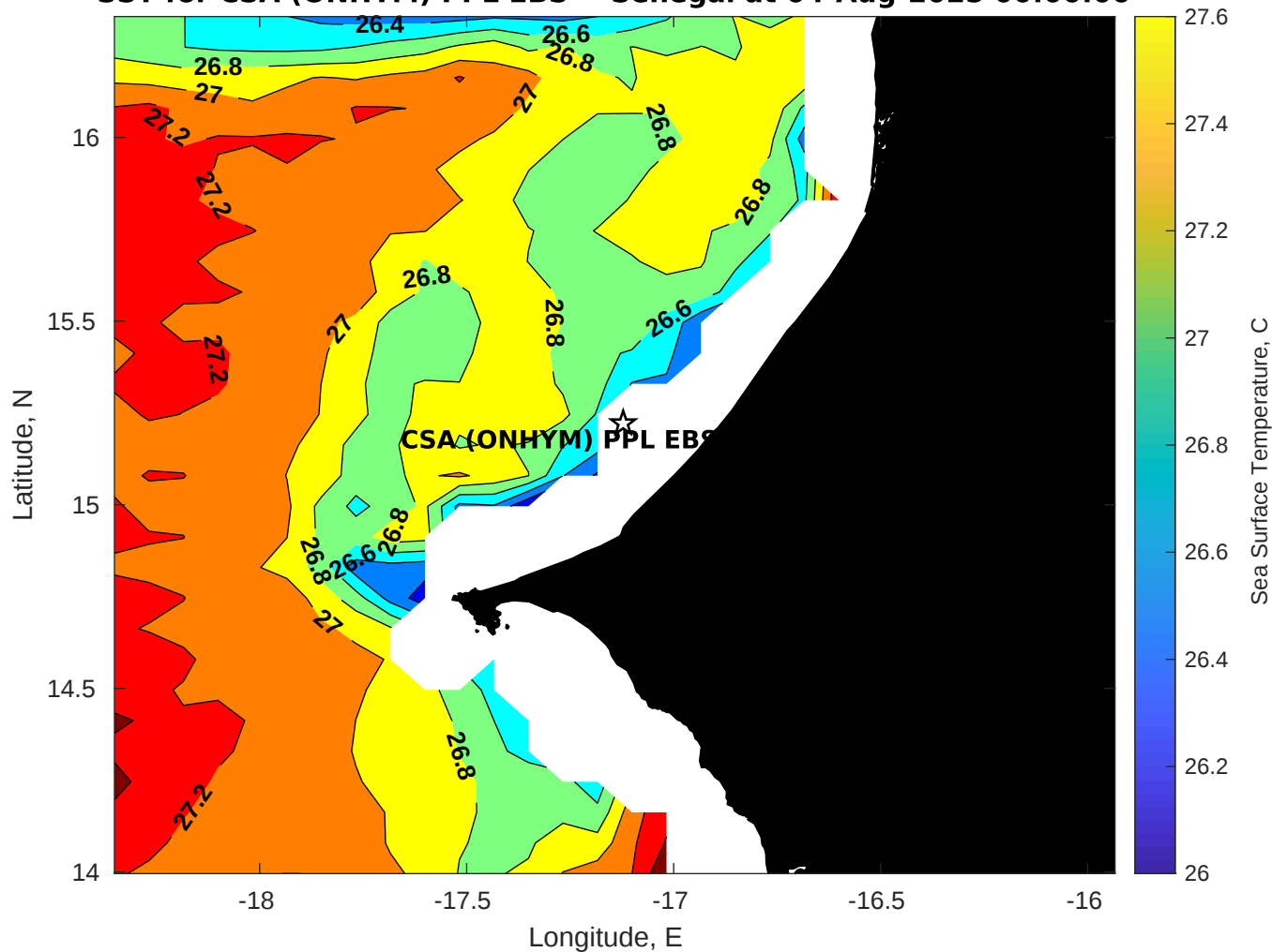
SST for CSA (ONHYM) PPL EBS - Senegal at 04-Aug-2025 00:00:00
