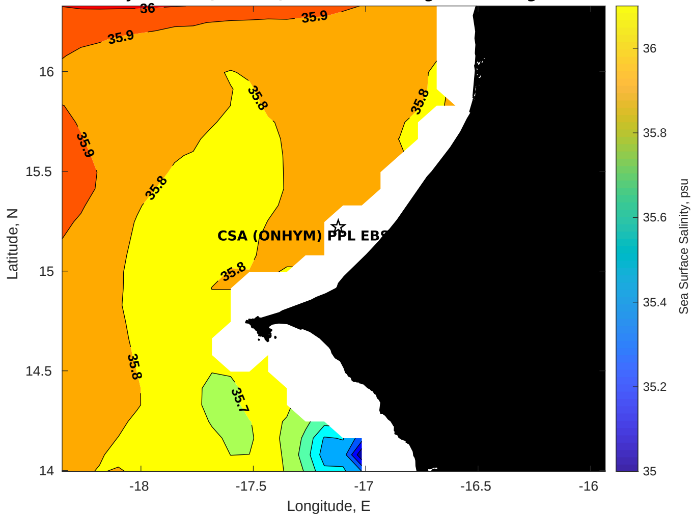
Surface Salinity for CSA (ONHYM) PPL EBS - Senegal at 04-Aug-2025 00:00:00
